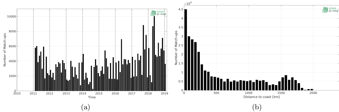
Figure 1: Number of match-ups between TSG (LEGOS-DM) and SMOS L3 v2 - 9-Days (BEC) SSS as a function of time (a) and as function of the distance to coast (b) over the Tropical Atlantic Ocean Pi-MEP region and for the full satellite product period.
