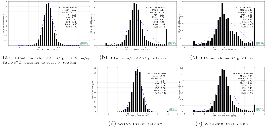
Figure 13: Normalized histogram of \Delta\text{SSS} (SMOS L3 v2 - 9-Days (BEC) - TSG (LEGOS-DM)) for 5 different subdatasets corresponding to: RR=0 mm/h, 3 < U_{10} < 12 m/s, SST>5°C, distance to coast > 800 km (a), RR=0 mm/h, 3 < U_{10} < 12 m/s (b), RR>1mm/h and U_{10} < 4 m/s (c), WOA2013 SSS Std<0.2 (d), WOA2013 SSS Std>0.2 (e).
