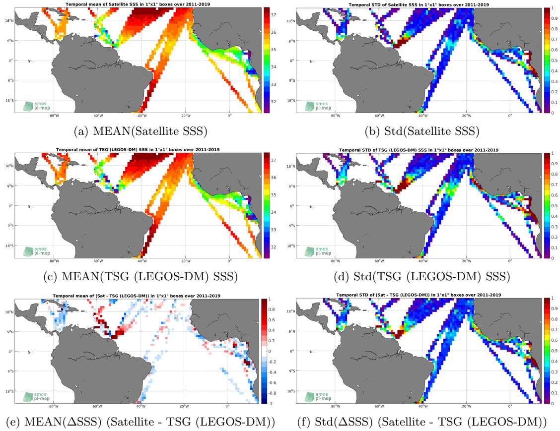
Figure 6: Temporal mean (left) and Std (right) of SSS from SMOS L3 v2 - 9-Days (BEC) (top), TSG (LEGOS-DM) (middle), and of \Delta SSS (Satellite - TSG (LEGOS-DM)). Only match-up pairs are used to generate these maps.
