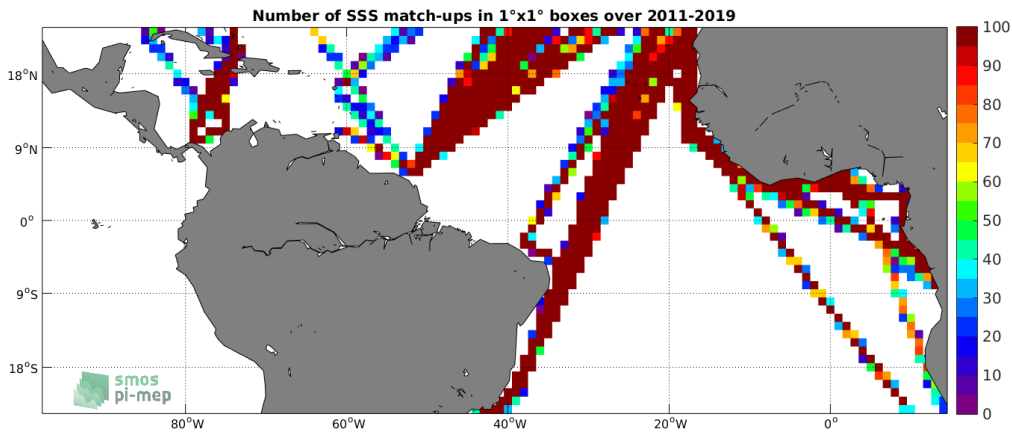
Figure 4: Number of SSS match-ups between TSG (LEGOS-DM) SSS and the SMOS L3 v2 - 9-Days (BEC) SSS product for the Tropical Atlantic Ocean Pi-MEP region over 1^\circ \times 1^\circ boxes and for the full satellite product period.
