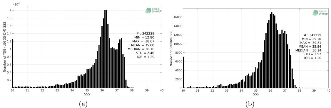
Figure 2: Histograms of SSS from TSG (LEGOS-DM) (a) and SMOS L3 v2 - 9-Days (BEC) (b) considering all match-up pairs per bins of 0.1 over the Tropical Atlantic Ocean Pi-MEP region and for the full satellite product period.
