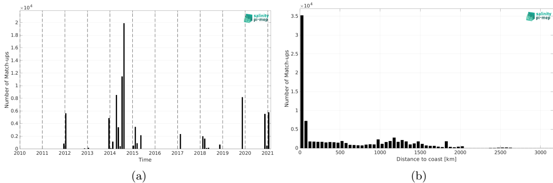
Figure 2: Number of match-ups between TSG (GOSUD-Sailing-ship) and SMOS SSS L3 v2 - 9-Days (BEC) SSS as a function of time (a) and as function of the distance to coast (b) over the Tropical Atlantic Ocean Pi-MEP region and for the full satellite product period.
