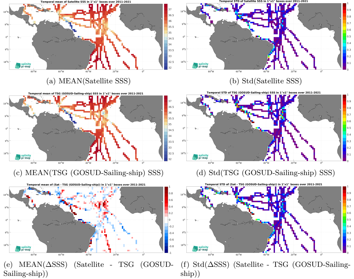
Figure 7: Temporal mean (left) and Std (right) of SSS from SMOS SSS L3 v2 - 9-Days (BEC) (top), TSG (GOSUD-Sailing-ship) (middle), and of \Delta\text{SSS} (Satellite - TSG (GOSUD-Sailing-ship)). Only match-up pairs are used to generate these maps.
