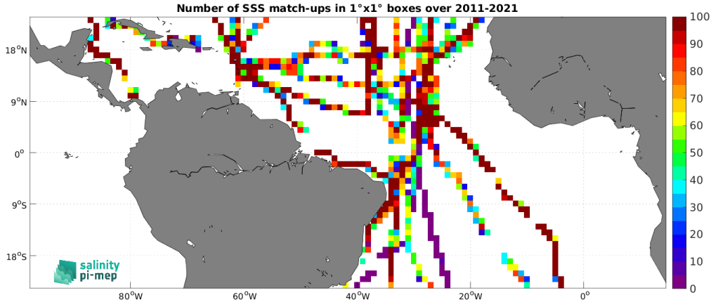
Figure 5: Number of SSS match-ups between TSG (GOSUD-Sailing-ship) SSS and the SMOS SSS L3 v2 - 9-Days (BEC) SSS product for the Tropical Atlantic Ocean Pi-MEP region over 1^\circ \times 1^\circ boxes and for the full satellite product period.
