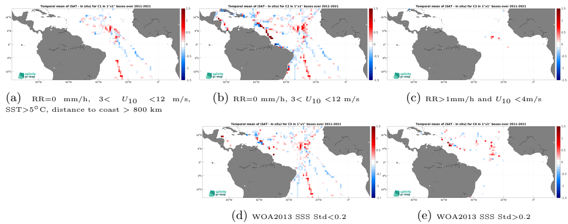
Figure 14: Temporal mean gridded over spatial boxes of size 1^\circ \times 1^\circ of \Delta\text{SSS} (SMOS SSS L3 v2 - 9-Days (BEC) - TSG (GOSUD-Sailing-ship)) for 5 different subdatasets corresponding to:RR=0 mm/h, 3 < U_{10} < 12 m/s, SST >5^\circ\text{C} , distance to coast > 800 km (a), RR=0 mm/h, 3 < U_{10} < 12 m/s (b), RR >1 mm/h and U_{10} < 4 m/s (c), WOA2013 SSS Std <0.2 (d), WOA2013 SSS Std >0.2 (e).
