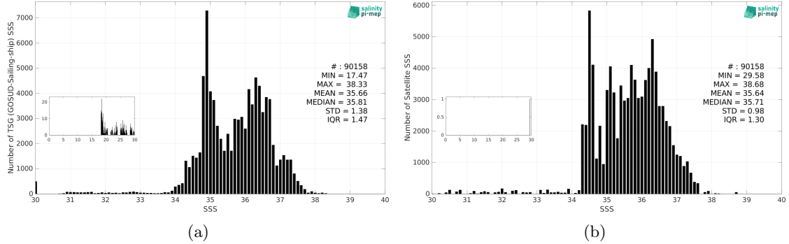
Figure 3: Histograms of SSS from TSG (GOSUD-Sailing-ship) (a) and SMOS SSS L3 v2 - 9-Days (BEC) (b) considering all match-up pairs per bins of 0.1 over the Tropical Atlantic Ocean Pi-MEP region and for the full satellite product period.
