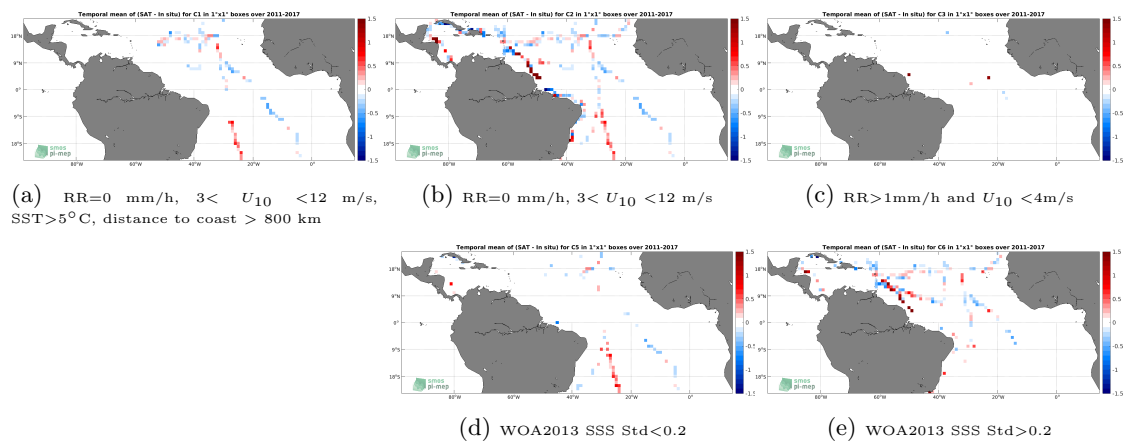
Figure 12: Temporal mean gridded over spatial boxes of size 1°x1° of \Delta SSS (SMOS SSS L3 v2 - 9-Days (BEC) - TSG (GOSUD-Sailing-ship)) for 5 different subdatasets corresponding to:RR=0 mm/h, 3 < U_{10} < 12 m/s, SST>5°C, distance to coast > 800 km (a), RR=0 mm/h, 3 < U_{10} < 12 m/s (b), RR>1mm/h and U_{10} < 4 m/s (c), WOA2013 SSS Std<0.2 (d), WOA2013 SSS Std>0.2 (e).
