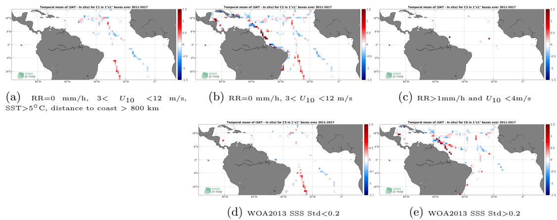
Figure 12: Temporal mean gridded over spatial boxes of size 1^\circ \times 1^\circ of \Delta\text{SSS} (SMOS L3 v2 - 9-Days (BEC) - TSG (GOSUD-Sailing-ship)) for 5 different subdatasets corresponding to: RR=0 mm/h, 3 < U_{10} < 12 m/s, SST > 5°C, distance to coast > 800 km (a), RR=0 mm/h, 3 < U_{10} < 12 m/s (b), RR > 1mm/h and U_{10} < 4 m/s (c), WOA2013 SSS Std < 0.2 (d), WOA2013 SSS Std > 0.2 (e).
