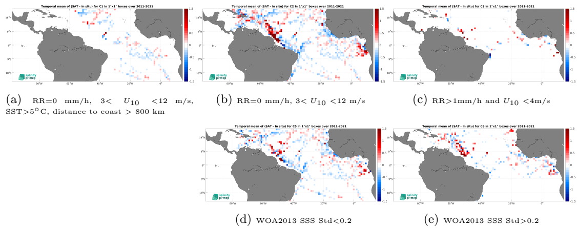
Figure 14: Temporal mean gridded over spatial boxes of size 1^\circ \times 1^\circ of \Delta\text{SSS} (SMOS SSS L3 v2 - 9-Days (BEC) - TSG (GOSUD-Research-vessel)) for 5 different subdatasets corresponding to:RR=0 mm/h, 3 < U_{10} < 12 m/s, SST>5°C, distance to coast > 800 km (a), RR=0 mm/h, 3 < U_{10} < 12 m/s (b), RR>1mm/h and U_{10} < 4 m/s (c), WOA2013 SSS Std<0.2 (d), WOA2013 SSS Std>0.2 (e).
