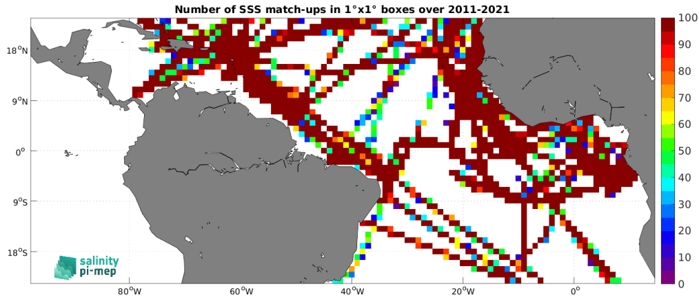
Figure 5: Number of SSS match-ups between TSG (GOSUD-Research-vessel) SSS and the SMOS SSS L3 v2 - 9-Days (BEC) SSS product for the Tropical Atlantic Ocean Pi-MEP region over 1^\circ \times 1^\circ boxes and for the full satellite product period.
