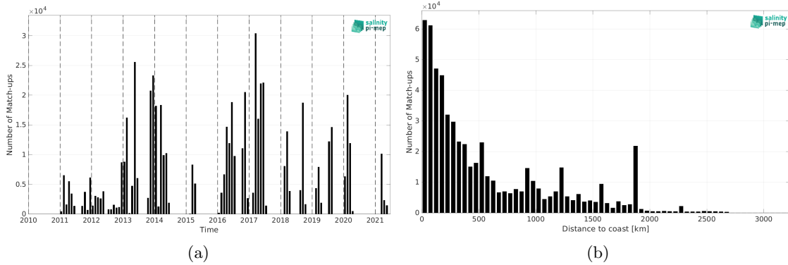
Figure 2: Number of match-ups between TSG (GOSUD-Research-vessel) and SMOS SSS L3 v2 - 9-Days (BEC) SSS as a function of time (a) and as function of the distance to coast (b) over the Tropical Atlantic Ocean Pi-MEP region and for the full satellite product period.
