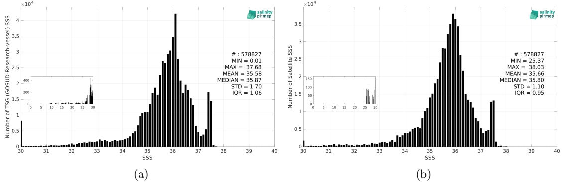
Figure 3: Histograms of SSS from TSG (GOSUD-Research-vessel) (a) and SMOS SSS L3 v2 - 9-Days (BEC) (b) considering all match-up pairs per bins of 0.1 over the Tropical Atlantic Ocean Pi-MEP region and for the full satellite product period.
