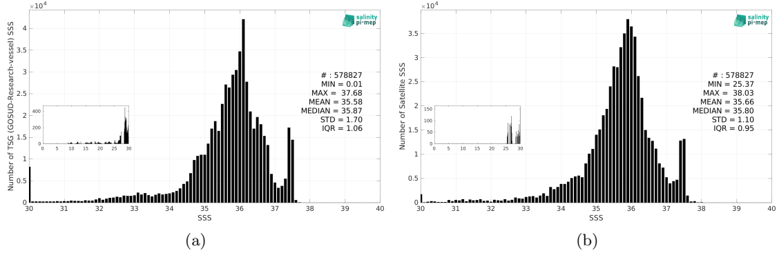
Figure 3: Histograms of SSS from TSG (GOSUD-Research-vessel) (a) and SMOS SSS L3 v2 - 9-Days (BEC) (b) considering all match-up pairs per bins of 0.1 over the Tropical Atlantic Ocean Pi-MEP region and for the full satellite product period.
