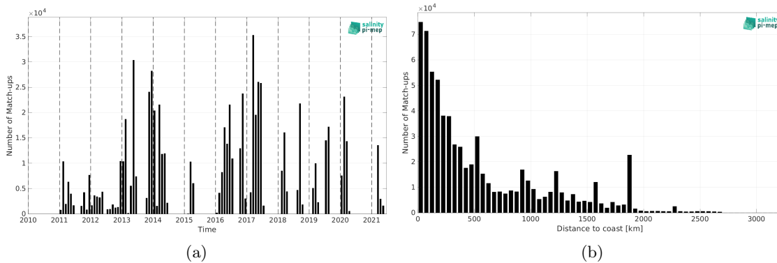
Figure 1: Number of match-ups between TSG (GOSUD-Research-vessel) and SMOS SSS L3 v2 - 9-Days (BEC) SSS as a function of time (a) and as function of the distance to coast (b) over the Tropical Atlantic Ocean Pi-MEP region and for the full satellite product period.
