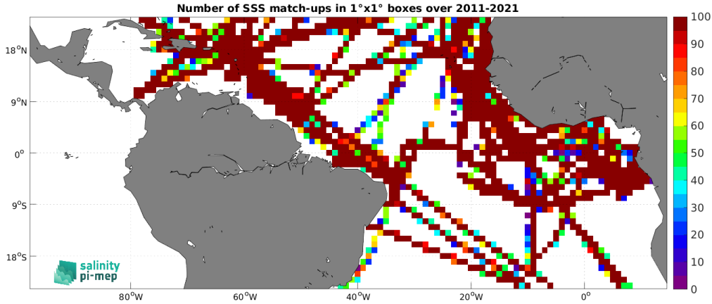
Figure 4: Number of SSS match-ups between TSG (GOSUD-Research-vessel) SSS and the SMOS SSS L3 v2 - 9-Days (BEC) SSS product for the Tropical Atlantic Ocean Pi-MEP region over 1^\circ \times 1^\circ boxes and for the full satellite product period.
