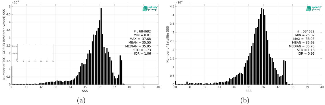
Figure 2: Histograms of SSS from TSG (GOSUD-Research-vessel) (a) and SMOS SSS L3 v2 - 9-Days (BEC) (b) considering all match-up pairs per bins of 0.1 over the Tropical Atlantic Ocean Pi-MEP region and for the full satellite product period.
