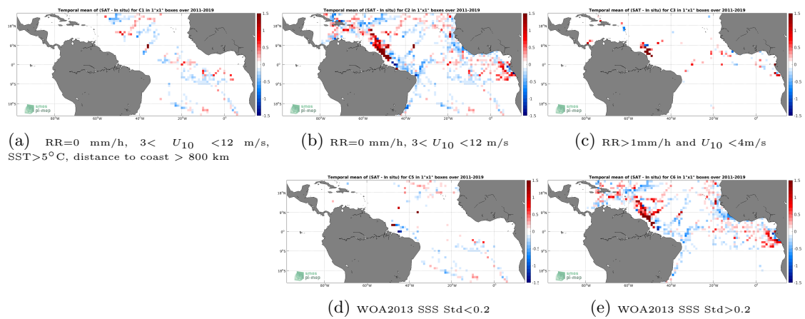
Figure 12: Temporal mean gridded over spatial boxes of size 1^\circ \times 1^\circ of \Delta\text{SSS} (SMOS SSS L3 v2 - 9-Days (BEC) - TSG (GOSUD-Research-vessel)) for 5 different subdatasets corresponding to:RR=0 mm/h, 3 < U_{10} < 12 m/s, SST>5°C, distance to coast > 800 km (a), RR=0 mm/h, 3 < U_{10} < 12 m/s (b), RR>1mm/h and U_{10} < 4 m/s (c), WOA2013 SSS Std<0.2 (d), WOA2013 SSS Std>0.2 (e).
