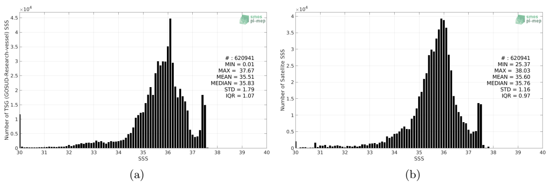
Figure 2: Histograms of SSS from TSG (GOSUD-Research-vessel) (a) and SMOS SSS L3 v2 - 9-Days (BEC) (b) considering all match-up pairs per bins of 0.1 over the Tropical Atlantic Ocean Pi-MEP region and for the full satellite product period.
