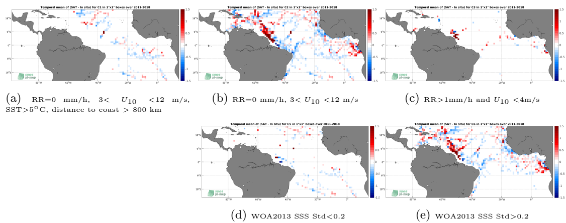
Figure 12: Temporal mean gridded over spatial boxes of size 1^\circ \times 1^\circ of \Delta\text{SSS} (SMOS L3 v2 - 9-Days (BEC) - TSG (GOSUD-Research-vessel)) for 5 different subdatasets corresponding to:RR=0 mm/h, 3 < U_{10} < 12 m/s, SST>5°C, distance to coast > 800 km (a), RR=0 mm/h, 3 < U_{10} < 12 m/s (b), RR>1mm/h and U_{10} < 4 m/s (c), WOA2013 SSS Std<0.2 (d), WOA2013 SSS Std>0.2 (e).
