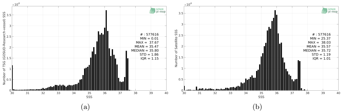
Figure 2: Histograms of SSS from TSG (GOSUD-Research-vessel) (a) and SMOS L3 v2 - 9-Days (BEC) (b) considering all match-up pairs per bins of 0.1 over the Tropical Atlantic Ocean Pi-MEP region and for the full satellite product period.
