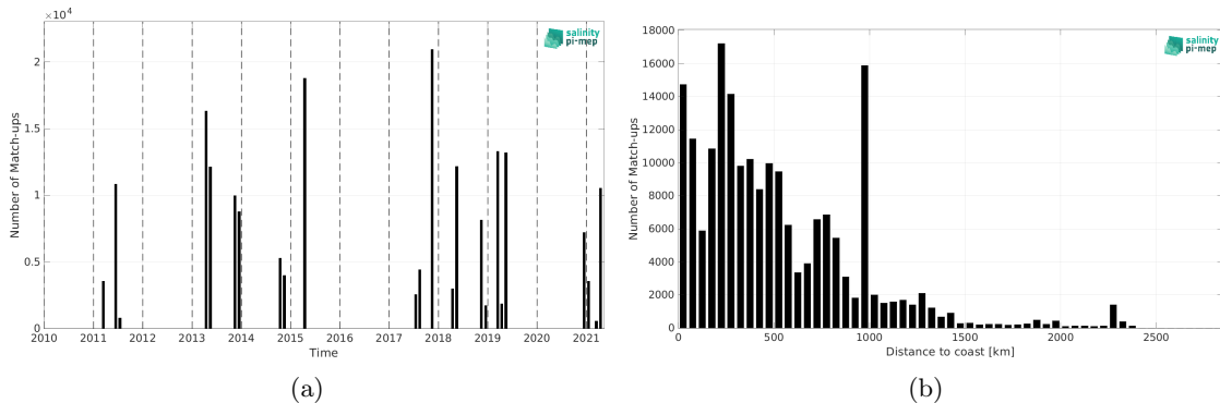
Figure 2: Number of match-ups between TSG (CSIC-UTM) and SMOS SSS L3 v2 - 9-Days (BEC) SSS as a function of time (a) and as function of the distance to coast (b) over the Tropical Atlantic Ocean Pi-MEP region and for the full satellite product period.
