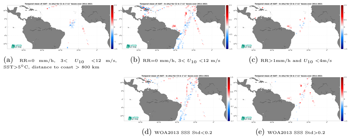
Figure 14: Temporal mean gridded over spatial boxes of size 1^\circ \times 1^\circ of \Delta\text{SSS} (SMOS SSS L3 v2 - 9-Days (BEC) - TSG (CSIC-UTM)) for 5 different subdatasets corresponding to:RR=0 mm/h, 3 < U_{10} < 12 m/s, SST >5^\circ\text{C} , distance to coast > 800 km (a), RR=0 mm/h, 3 < U_{10} < 12 m/s (b), RR >1 mm/h and U_{10} < 4 m/s (c), WOA2013 SSS Std <0.2 (d), WOA2013 SSS Std >0.2 (e).
