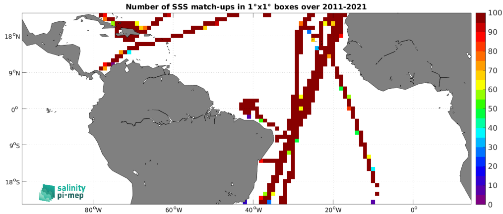
Figure 5: Number of SSS match-ups between TSG (CSIC-UTM) SSS and the SMOS SSS L3 v2 - 9-Days (BEC) SSS product for the Tropical Atlantic Ocean Pi-MEP region over 1^\circ \times 1^\circ boxes and for the full satellite product period.
