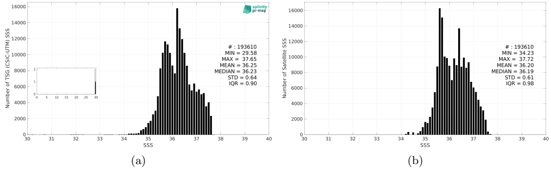
Figure 3: Histograms of SSS from TSG (CSIC-UTM) (a) and SMOS SSS L3 v2 - 9-Days (BEC) (b) considering all match-up pairs per bins of 0.1 over the Tropical Atlantic Ocean Pi-MEP region and for the full satellite product period.
