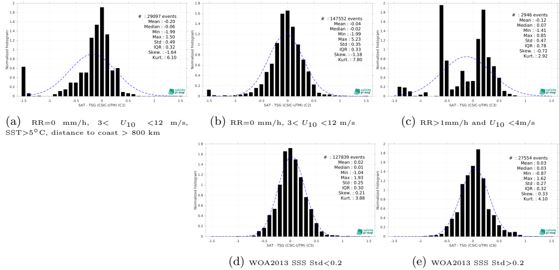
Figure 15: Normalized histogram of \Delta SSS (SMOS SSS L3 v2 - 9-Days (BEC) - TSG (CSIC-UTM)) for 5 different subdatasets corresponding to: RR=0 mm/h, 3 < U_{10} < 12 m/s, SST > 5°C, distance to coast > 800 km (a), RR=0 mm/h, 3 < U_{10} < 12 m/s (b), RR > 1mm/h and U_{10} < 4 m/s (c), WOA2013 SSS Std < 0.2 (d), WOA2013 SSS Std > 0.2 (e).
