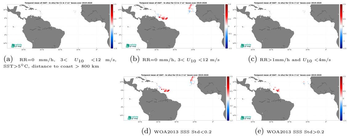
Figure 12: Temporal mean gridded over spatial boxes of size 1^\circ \times 1^\circ of \Delta\text{SSS} (SMOS SSS L3 v2 - 9-Days (BEC) - Saldrone) for 5 different subdatasets corresponding to:RR=0 mm/h, 3 < U_{10} < 12 m/s, SST >5^\circ\text{C} , distance to coast > 800 km (a), RR=0 mm/h, 3 < U_{10} < 12 m/s (b), RR >1 mm/h and U_{10} < 4 m/s (c), WOA2013 SSS Std <0.2 (d), WOA2013 SSS Std >0.2 (e).
