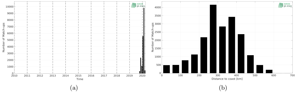
Figure 1: Number of match-ups between Saildrone and SMOS SSS L3 v2 - 9-Days (BEC) SSS as a function of time (a) and as function of the distance to coast (b) over the Tropical Atlantic Ocean Pi-MEP region and for the full satellite product period.
