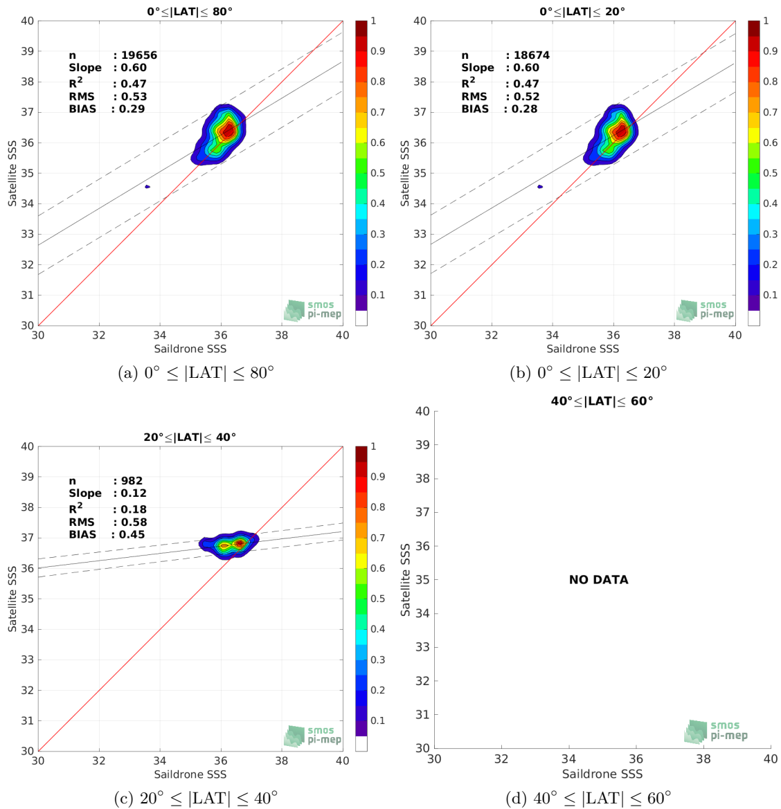
Figure 9: Contour maps of the concentration of SMOS SSS L3 v2 - 9-Days (BEC) SSS (y-axis) versus Saïldrone SSS (x-axis) at match-up pairs for different latitude bands. For each plot, the red line shows x=y . The black thin and dashed lines indicate a linear fit through the data cloud and the \pm 95\% confidence levels, respectively. The number match-up pairs n , the slope and R^2 coefficient of the linear fit, the root mean square (RMS) and the mean bias between satellite and in situ data are indicated for each latitude band in each plots.
