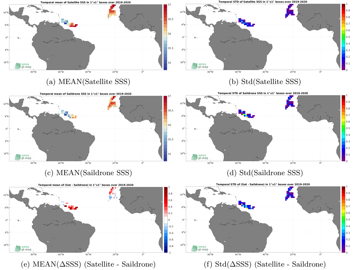
Figure 6: Temporal mean (left) and Std (right) of SSS from SMOS SSS L3 v2 - 9-Days (BEC) (top), Saildrone (middle), and of \Delta\text{SSS} (Satellite - Saildrone). Only match-up pairs are used to generate these maps.
