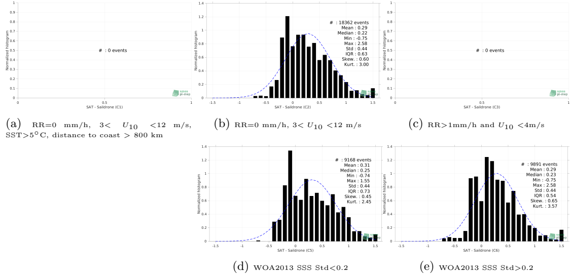
Figure 13: Normalized histogram of \Delta SSS (SMOS SSS L3 v2 - 9-Days (BEC) - Saildrone) for 5 different subdatasets corresponding to: RR=0 mm/h, 3 < U_{10} < 12 m/s, SST > 5°C, distance to coast > 800 km (a), RR=0 mm/h, 3 < U_{10} < 12 m/s (b), RR > 1mm/h and U_{10} < 4 m/s (c), WOA2013 SSS Std < 0.2 (d), WOA2013 SSS Std > 0.2 (e).
