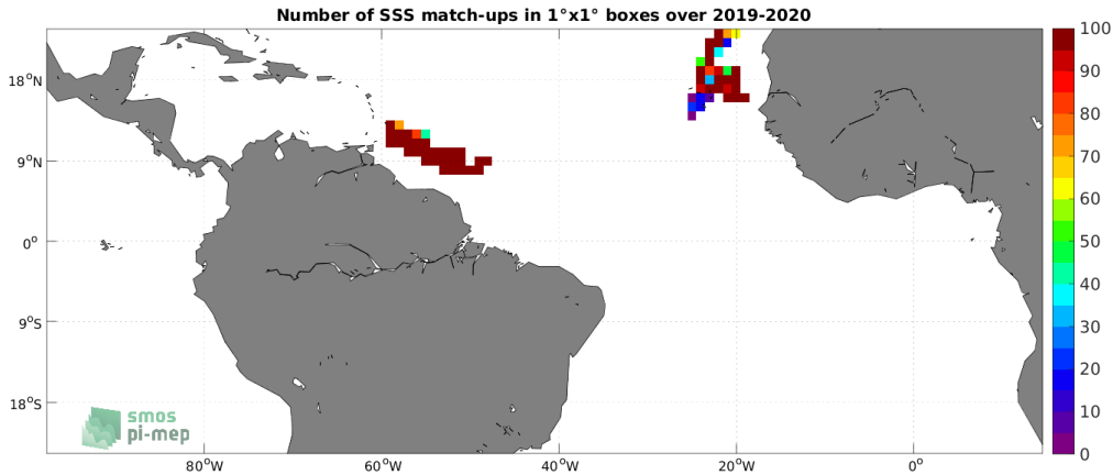
Figure 4: Number of SSS match-ups between Saildrone SSS and the SMOS SSS L3 v2 - 9-Days (BEC) SSS product for the Tropical Atlantic Ocean Pi-MEP region over 1^\circ \times 1^\circ boxes and for the full satellite product period.
