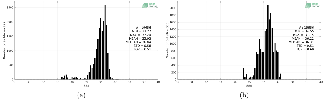
Figure 2: Histograms of SSS from Saildrone (a) and SMOS SSS L3 v2 - 9-Days (BEC) (b) considering all match-up pairs per bins of 0.1 over the Tropical Atlantic Ocean Pi-MEP region and for the full satellite product period.
