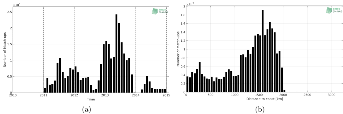
Figure 1: Number of match-ups between Surface drifters and SMOS L3 v2 - 9-Days (BEC) SSS as a function of time (a) and as function of the distance to coast (b) over the Tropical Atlantic Ocean Pi-MEP region and for the full satellite product period.
