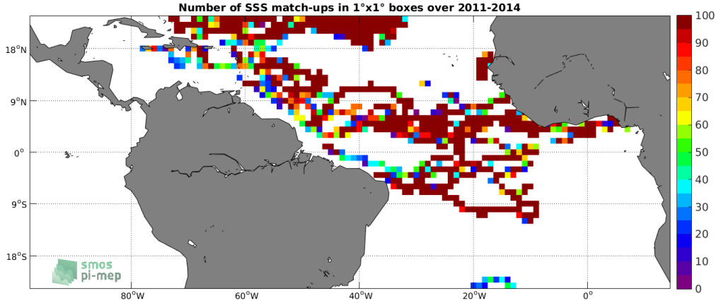
Figure 3: Number of SSS match-ups between Surface drifters SSS and the SMOS L3 v2 - 9-Days (BEC) SSS product for the Tropical Atlantic Ocean Pi-MEP region over 1^\circ \times 1^\circ boxes and for the full satellite product period.
