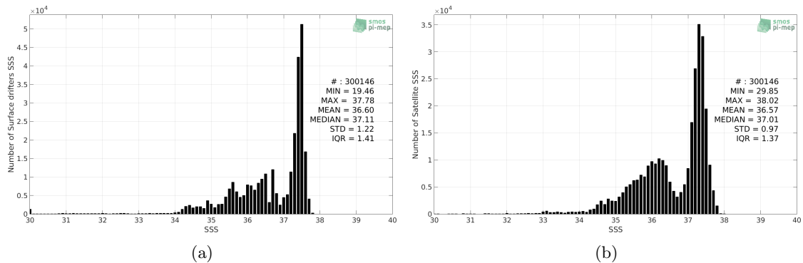
Figure 2: Histograms of SSS from Surface drifters (a) and SMOS L3 v2 - 9-Days (BEC) (b) considering all match-up pairs per bins of 0.1 over the Tropical Atlantic Ocean Pi-MEP region and for the full satellite product period.
