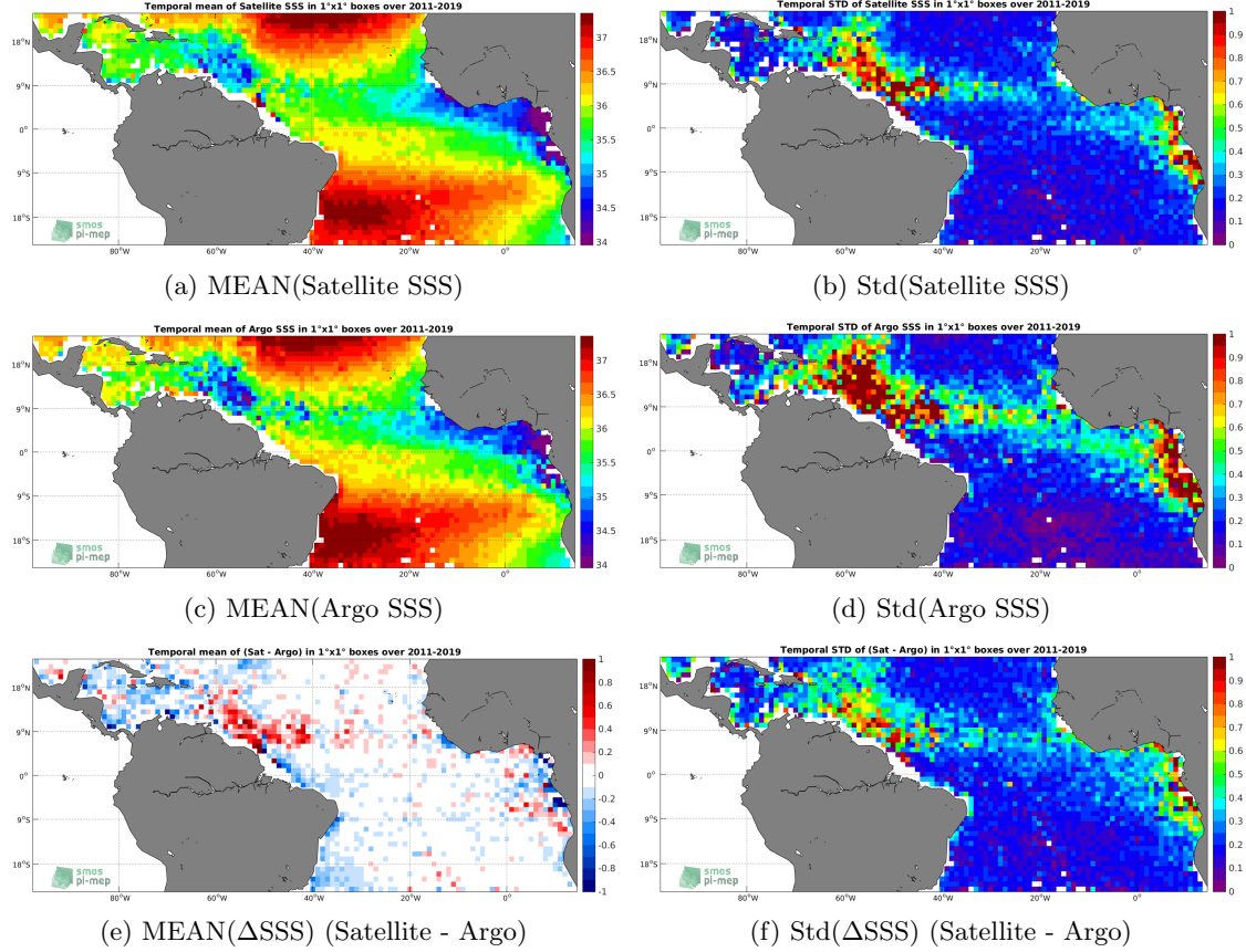
Figure 6: Temporal mean (left) and Std (right) of SSS from SMOS SSS L3 v2 - 9-Days (BEC) (top), Argo (middle), and of \Delta\text{SSS} (Satellite - Argo). Only match-up pairs are used to generate these maps.
