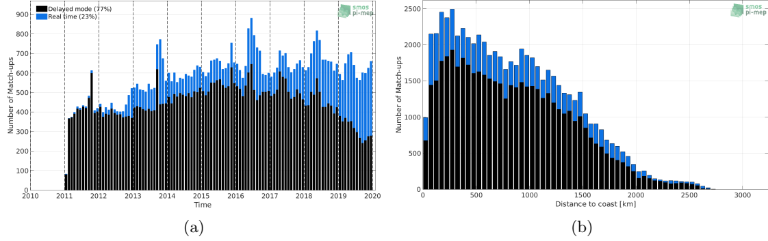
Figure 1: Number of match-ups between Argo and SMOS L3 v2 - 9-Days (BEC) SSS as a function of time (a) and as function of the distance to coast (b) over the Tropical Atlantic Ocean Pi-MEP region and for the full satellite product period.
