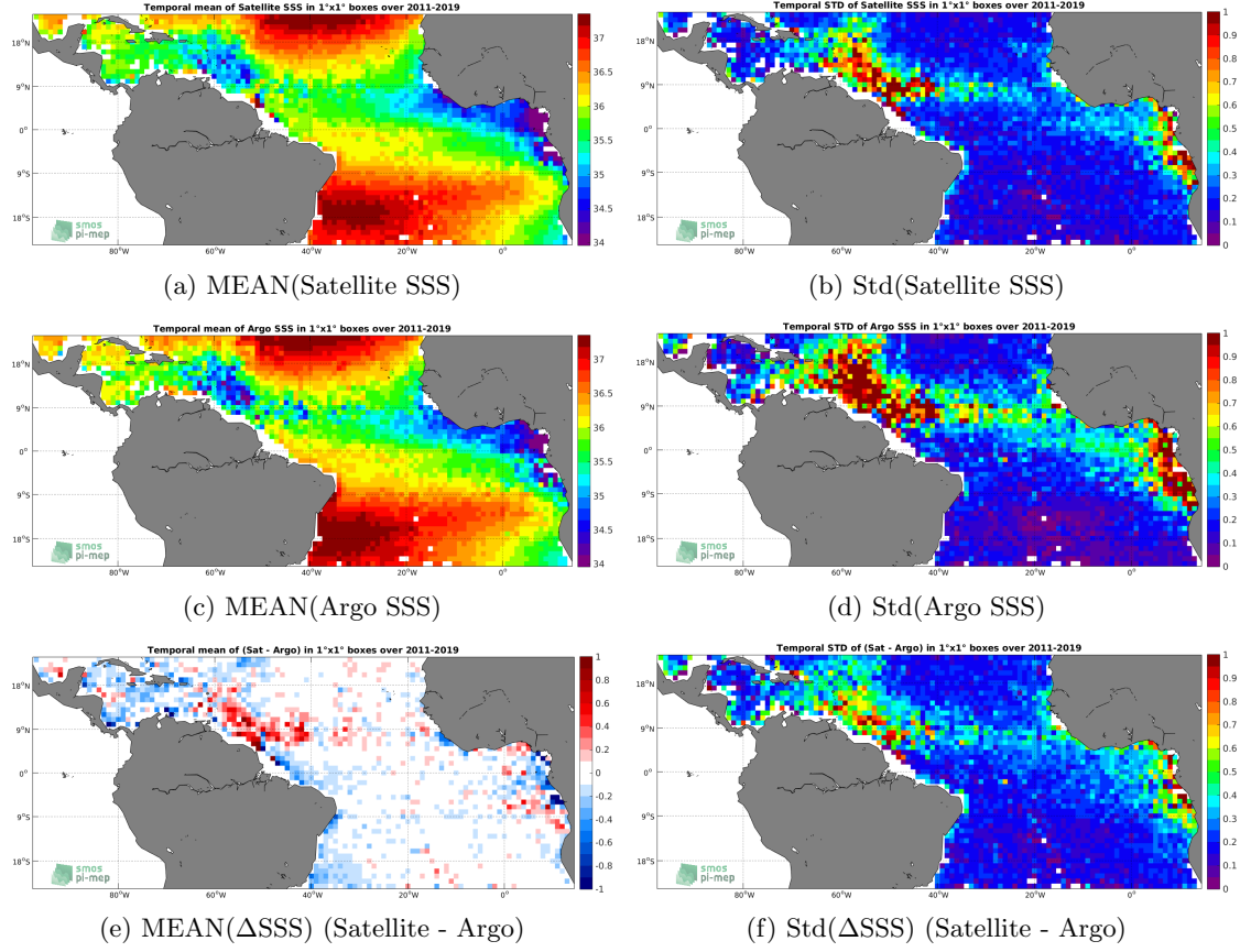
Figure 6: Temporal mean (left) and Std (right) of SSS from SMOS L3 v2 - 9-Days (BEC) (top), Argo (middle), and of \Delta SSS (Satellite - Argo). Only match-up pairs are used to generate these maps.
