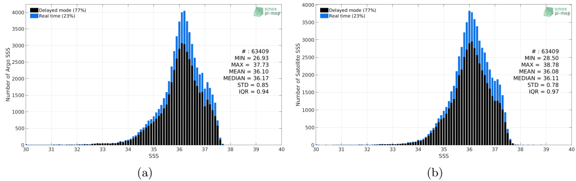
Figure 2: Histograms of SSS from Argo (a) and SMOS L3 v2 - 9-Days (BEC) (b) considering all match-up pairs per bins of 0.1 over the Tropical Atlantic Ocean Pi-MEP region and for the full satellite product period.
