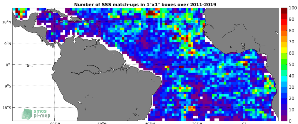
Figure 4: Number of SSS match-ups between Argos SSS and the SMOS L3 v2 - 9-Days (BEC) SSS product for the Tropical Atlantic Ocean Pi-MEP region over 1°x1° boxes and for the full satellite product period.
