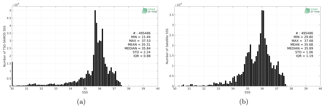
Figure 2: Histograms of SSS from TSG-SAMOS (a) and SMOS-L3-BEC-OA-V1-9DAYS-0.25DEG (b) considering all match-up pairs per bins of 0.1 over the Tropical Atlantic Ocean Pi-MEP region and for the full satellite product period.
