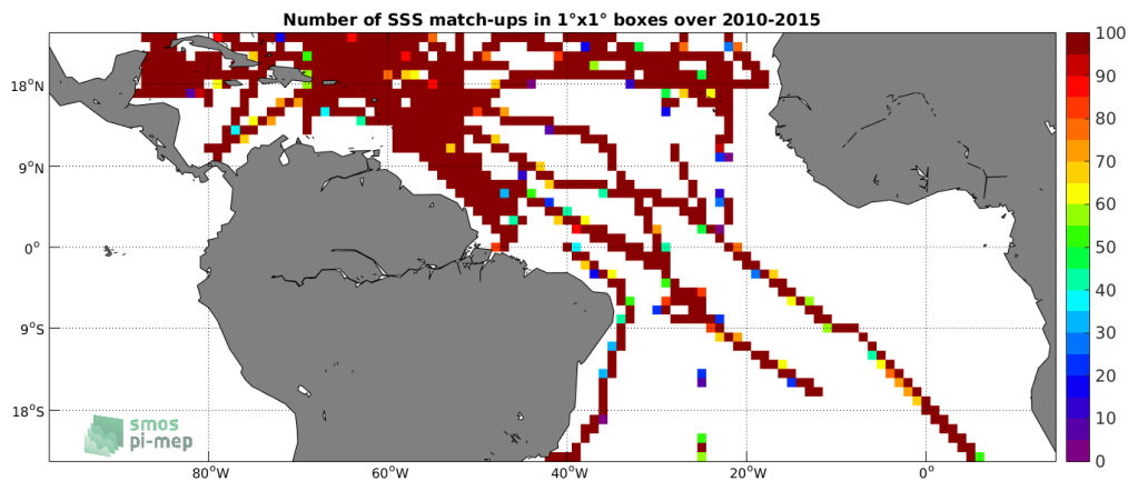
Figure 4: Number of SSS match-ups between TSG-SAMOS SSS and the SMOS-L3-BEC-OA-V1-9DAYS-0.25DEG SSS product for the Tropical Atlantic Ocean Pi-MEP region over 1^\circ \times 1^\circ boxes and for the full satellite product period.
