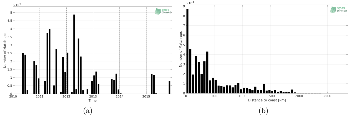
Figure 1: Number of match-ups between TSG-SAMOS and SMOS-L3-BEC-OA-V1-9DAYS-0.25DEG SSS as a function of time (a) and as function of the distance to coast (b) over the Tropical Atlantic Ocean Pi-MEP region and for the full satellite product period.
