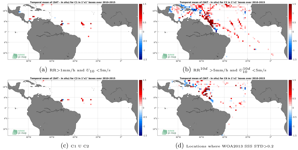
Figure 12: Temporal mean gridded over spatial boxes of size 1^\circ \times 1^\circ of \Delta SSS (SMOS-L3-BEC-OA-V1-9DAYS-0.25DEG - TSG-SAMOS) for 4 different subdatasets corresponding to: RR > 1mm/h and U_{10} < 5\text{m/s} (a), RR^{10d} > 5\text{mm/h} and U_{10}^{10d} < 5\text{m/s} (b), C1 U C2 (c), Locations where WOA2013 SSS STD > 0.2 (d).
