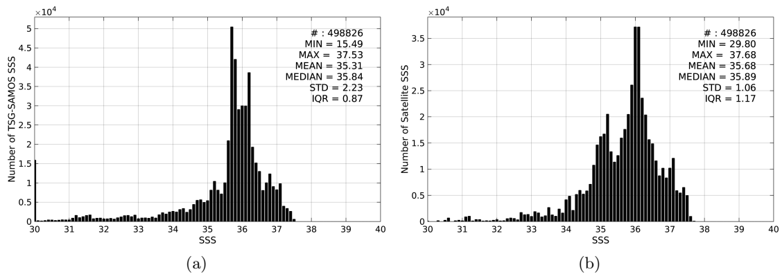
Figure 2: Histograms of SSS from TSG-SAMOS (a) and SMOS-L3-BEC-OA-V1-9DAYS-0.25DEG (b) considering all match-up pairs per bins of 0.1 over the Tropical Atlantic Ocean Pi-MEP region and for the full satellite product period.
