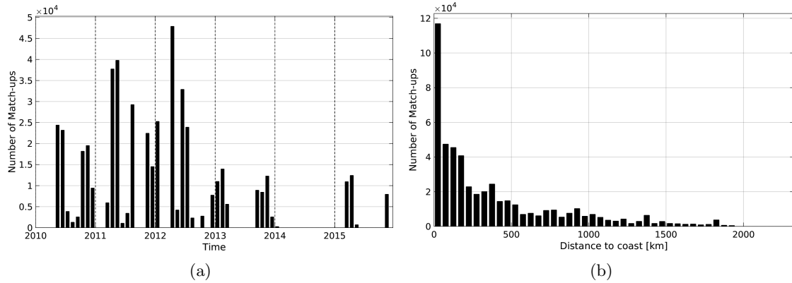
Figure 1: Number of match-ups between TSG-SAMOS and SMOS-L3-BEC-OA-V1-9DAYS-0.25DEG SSS as a function of time (a) and as function of the distance to coast (b) over the Tropical Atlantic Ocean Pi-MEP region and for the full satellite product period.
