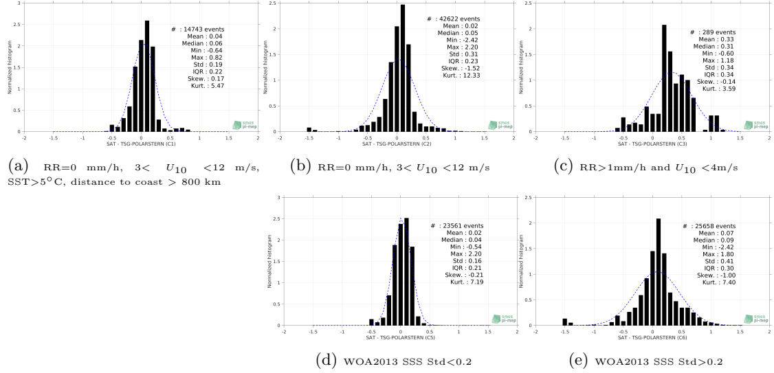
Figure 13: Normalized histogram of \Delta SSS (SMOS-L3-BEC-OA-V1-9DAYS-0.25DEG - TSG-POLARSTERN) for 5 different subdatasets corresponding to: RR=0 mm/h, 3 < U_{10} < 12 m/s, SST > 5°C, distance to coast > 800 km (a), RR=0 mm/h, 3 < U_{10} < 12 m/s (b), RR > 1mm/h and U_{10} < 4 m/s (c), WOA2013 SSS Std < 0.2 (d), WOA2013 SSS Std > 0.2 (e).
