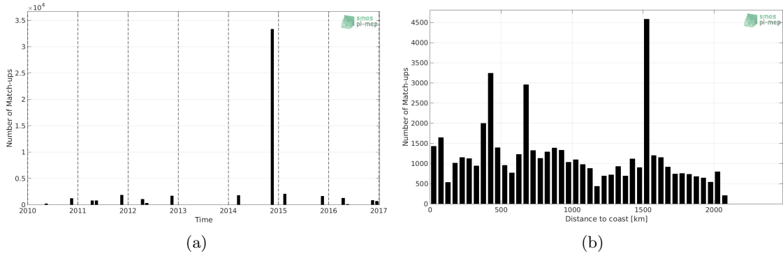
Figure 1: Number of match-ups between TSG-POLARSTERN and SMOS-L3-BEC-OA-V1-9DAYS-0.25DEG SSS as a function of time (a) and as function of the distance to coast (b) over the Tropical Atlantic Ocean Pi-MEP region and for the full satellite product period.
