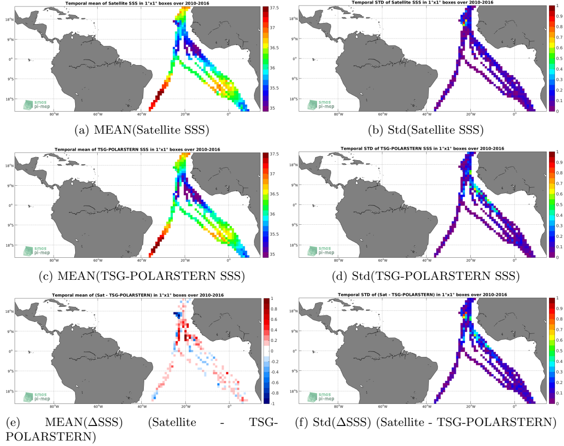
Figure 6: Temporal mean (left) and Std (right) of SSS from SMOS-L3-BEC-OA-V1-9DAYS-0.25DEG (top), TSG-POLARSTERN (middle), and of \Delta SSS (Satellite - TSG-POLARSTERN). Only match-up pairs are used to generate these maps.
