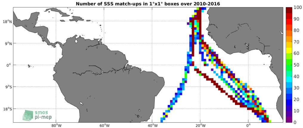
Figure 4: Number of SSS match-ups between TSG-POLARSTERN SSS and the SMOS-L3-BEC-OA-V1-9DAYS-0.25DEG SSS product for the Tropical Atlantic Ocean Pi-MEP region over 1^\circ \times 1^\circ boxes and for the full satellite product period.
