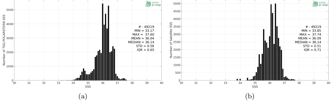
Figure 2: Histograms of SSS from TSG-POLARSTERN (a) and SMOS-L3-BEC-OA-V1-9DAYS-0.25DEG (b) considering all match-up pairs per bins of 0.1 over the Tropical Atlantic Ocean Pi-MEP region and for the full satellite product period.
