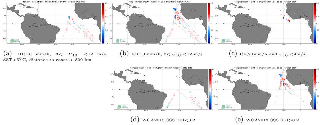
Figure 12: Temporal mean gridded over spatial boxes of size 1^\circ \times 1^\circ of \Delta SSS (SMOS-L3-BEC-OA-V1-9DAYS-0.25DEG - TSG-POLARSTERN) for 5 different subdatasets corresponding to:RR=0 mm/h, 3 < U_{10} < 12 m/s, SST >5^\circ\text{C} , distance to coast > 800 km (a), RR=0 mm/h, 3 < U_{10} < 12 m/s (b), RR >1 mm/h and U_{10} < 4 m/s (c), WOA2013 SSS Std <0.2 (d), WOA2013 SSS Std >0.2 (e).
