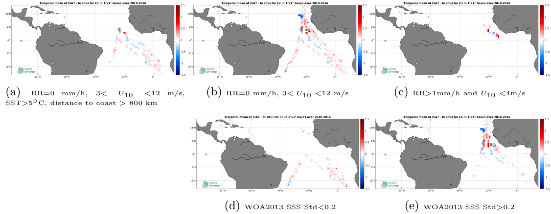
Figure 12: Temporal mean gridded over spatial boxes of size 1^\circ \times 1^\circ of \Delta SSS (SMOS-L3-BEC-OA-V1-9DAYS-0.25DEG - TSG-POLARSTERN) for 5 different subdatasets corresponding to: RR=0 mm/h, 3 < U_{10} < 12 m/s, SST > 5^\circ C , distance to coast > 800 km (a), RR=0 mm/h, 3 < U_{10} < 12 m/s (b), RR > 1 mm/h and U_{10} < 4 m/s (c), WOA2013 SSS Std < 0.2 (d), WOA2013 SSS Std > 0.2 (e).
