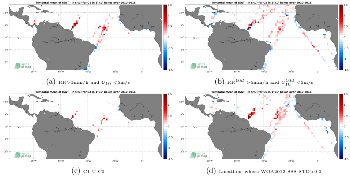
Figure 12: Temporal mean gridded over spatial boxes of size 1^\circ \times 1^\circ of \Delta\text{SSS} (SMOS-L3-BEC-OA-V1-9DAYS-0.25DEG - TSG-LEGOS-DM) for 4 different subdatasets corresponding to: RR > 1\text{mm/h} and U_{10} < 5\text{m/s} (a), RR^{10d} > 5\text{mm/h} and U_{10}^{10d} < 5\text{m/s} (b), C1 U C2 (c), Locations where WOA2013 SSS STD > 0.2 (d).
