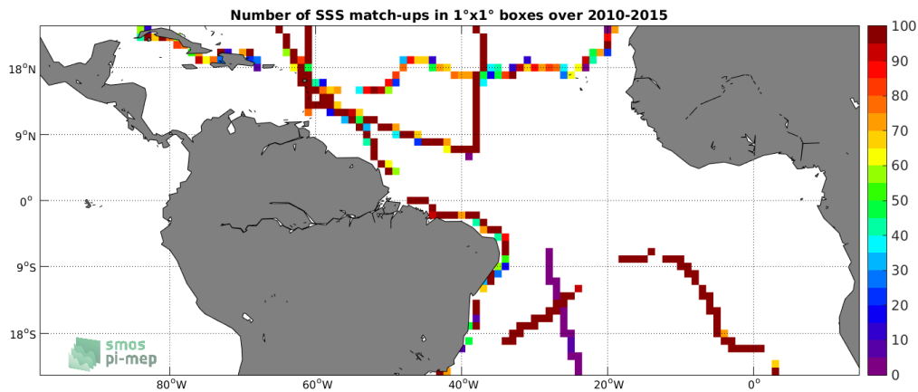
Figure 4: Number of SSS match-ups between TSG-GOSUD-Sailing-ship SSS and the SMOS-L3-BEC-OA-V1-9DAYS-0.25DEG SSS product for the Tropical Atlantic Ocean Pi-MEP region over 1^\circ \times 1^\circ boxes and for the full satellite product period.
