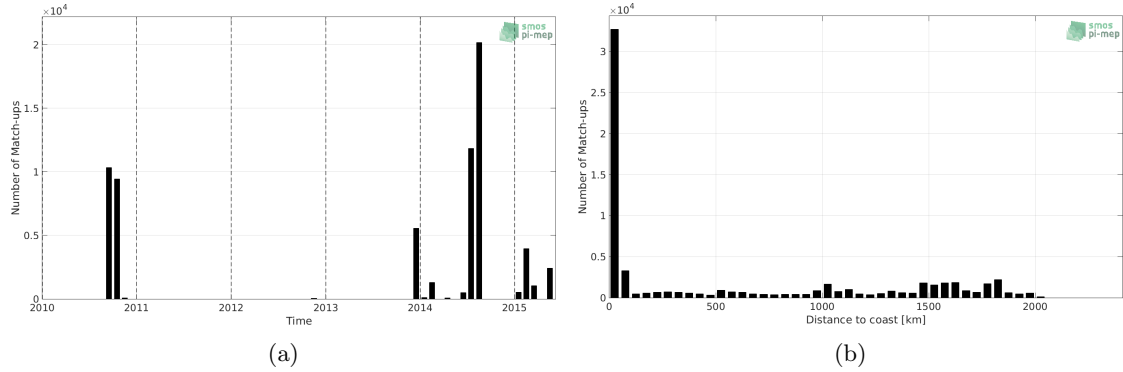
Figure 1: Number of match-ups between TSG-GOSUD-Sailing-ship and SMOS-L3-BEC-OA-V1-9DAYS-0.25DEG SSS as a function of time (a) and as function of the distance to coast (b) over the Tropical Atlantic Ocean Pi-MEP region and for the full satellite product period.
