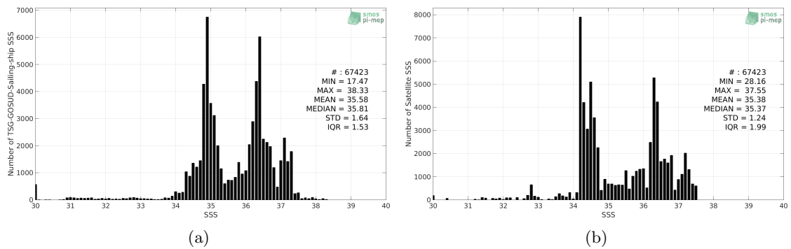
Figure 2: Histograms of SSS from TSG-GOSUD-Sailing-ship (a) and SMOS-L3-BEC-OA-V1-9DAYS-0.25DEG (b) considering all match-up pairs per bins of 0.1 over the Tropical Atlantic Ocean Pi-MEP region and for the full satellite product period.
