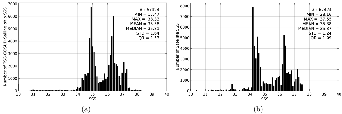
Figure 2: Histograms of SSS from TSG-GOSUD-Sailing-ship (a) and SMOS-L3-BEC-OA-V1-9DAYS-0.25DEG (b) considering all match-up pairs per bins of 0.1 over the Tropical Atlantic Ocean Pi-MEP region and for the full satellite product period.
