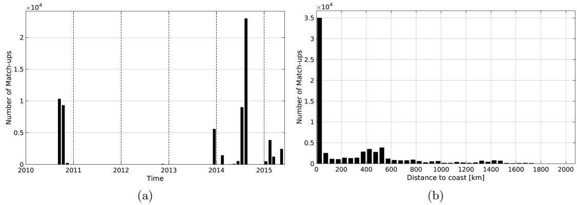
Figure 1: Number of match-ups between TSG-GOSUD-Sailing-ship and SMOS-L3-BEC-OA-V1-9DAYS-0.25DEG SSS as a function of time (a) and as function of the distance to coast (b) over the Tropical Atlantic Ocean Pi-MEP region and for the full satellite product period.
