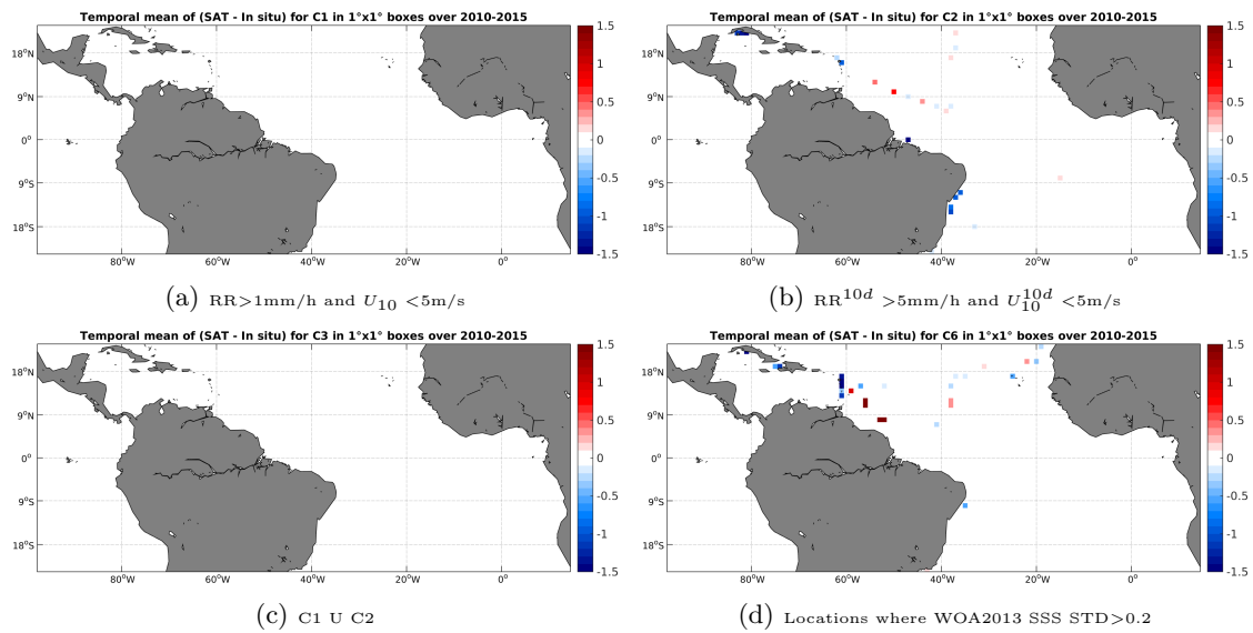
Figure 12: Temporal mean gridded over spatial boxes of size 1^\circ \times 1^\circ of \Delta SSS (SMOS-L3-BEC-OA-V1-9DAYS-0.25DEG - TSG-GOSUD-Sailing-ship) for 4 different subdatasets corresponding to:RR > 1 mm/h and U_{10} < 5 m/s (a), RR^{10d} > 5 mm/h and U_{10}^{10d} < 5 m/s (b), C1 U C2 (c),Locations where WOA2013 SSS STD > 0.2 (d).
