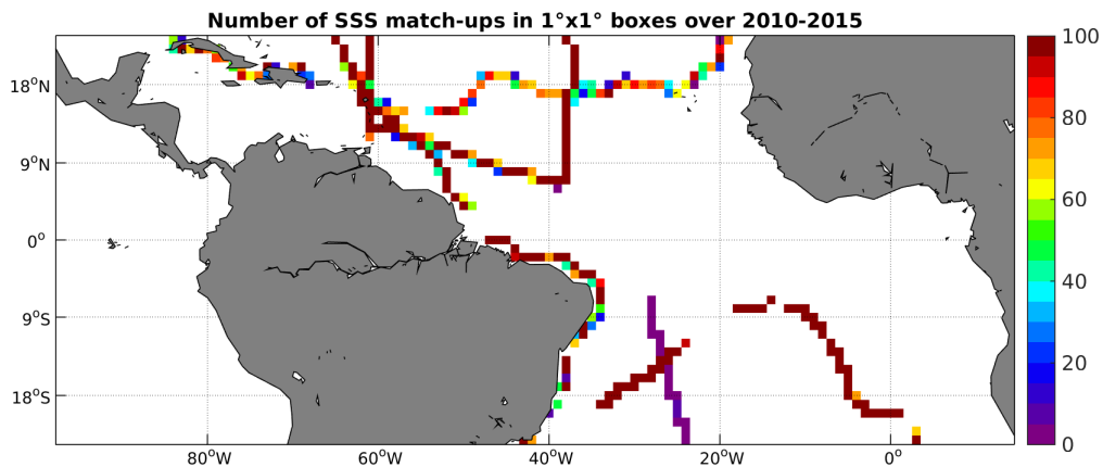
Figure 4: Number of SSS match-ups between TSG-GOSUD-Sailing-ship SSS and the SMOS-L3-BEC-OA-V1-9DAYS-0.25DEG SSS product for the Tropical Atlantic Ocean Pi-MEP region over 1°x1° boxes and for the full satellite product period.
