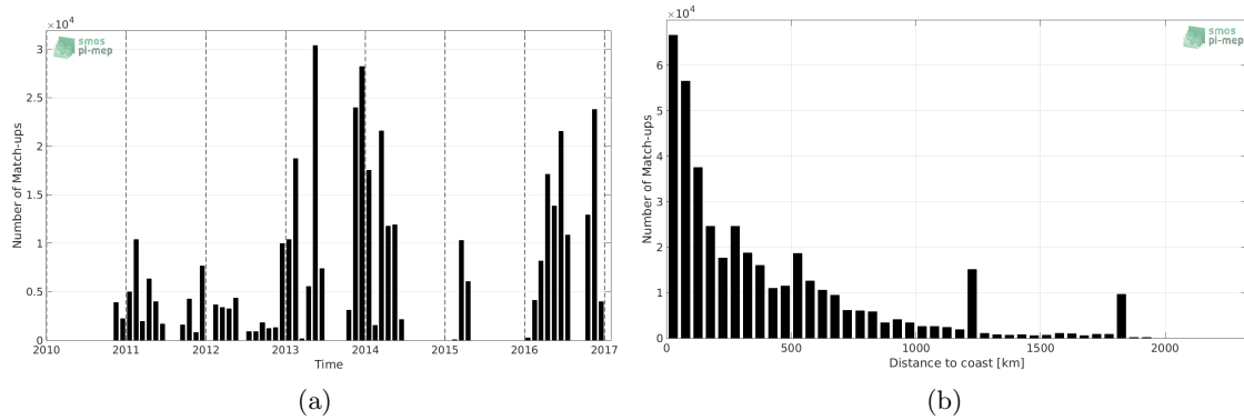
Figure 1: Number of match-ups between TSG-GOSUD-Research-vessel and SMOS-L3-BEC-OA-V1-9DAYS-0.25DEG SSS as a function of time (a) and as function of the distance to coast (b) over the Tropical Atlantic Ocean Pi-MEP region and for the full satellite product period.
