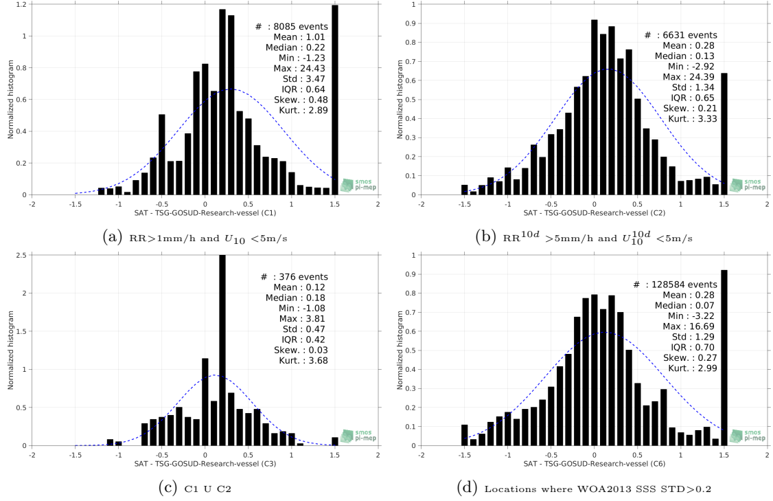
Figure 13: Normalized histogram of \Delta SSS (SMOS-L3-BEC-OA-V1-9DAYS-0.25DEG - TSG-GOSUD-Research-vessel) for 6 different subdatasets corresponding to: RR > 1mm/h and U_{10} < 5 m/s (a), RR^{10d} > 5 mm/h and U_{10}^{10d} < 5 m/s (b), C1 U C2 (c), Locations where WOA2013 SSS STD > 0.2 (d).
