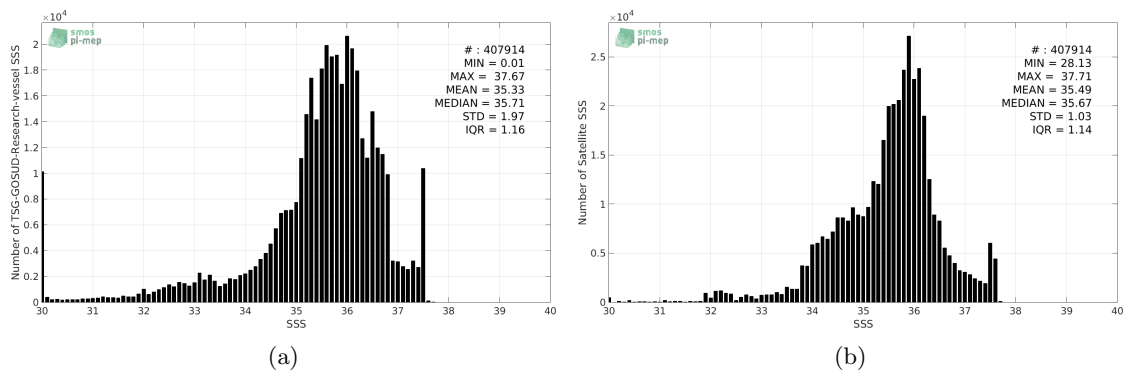
Figure 2: Histograms of SSS from TSG-GOSUD-Research-vessel (a) and SMOS-L3-BEC-OA-V1-9DAYS-0.25DEG (b) considering all match-up pairs per bins of 0.1 over the Tropical Atlantic Ocean Pi-MEP region and for the full satellite product period.
