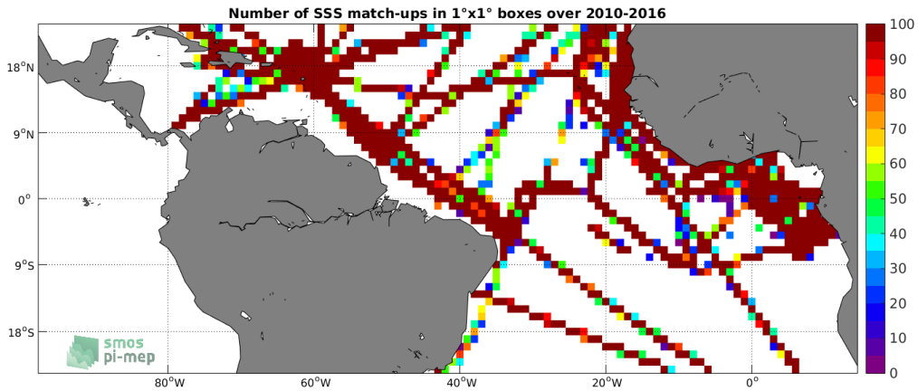
Figure 4: Number of SSS match-ups between TSG-GOSUD-Research-vessel SSS and the SMOS-L3-BEC-OA-V1-9DAYS-0.25DEG SSS product for the Tropical Atlantic Ocean Pi-MEP region over 1^\circ \times 1^\circ boxes and for the full satellite product period.
