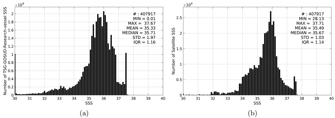
Figure 2: Histograms of SSS from TSG-GOSUD-Research-vessel (a) and SMOS-L3-BEC-OA-V1-9DAYS-0.25DEG (b) considering all match-up pairs per bins of 0.1 over the Tropical Atlantic Ocean Pi-MEP region and for the full satellite product period.
