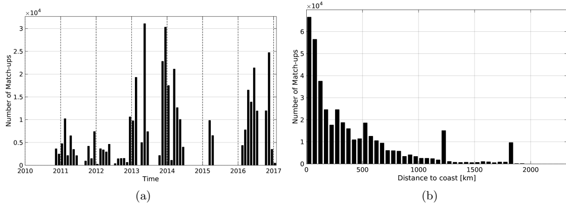
Figure 1: Number of match-ups between TSG-GOSUD-Research-vessel and SMOS-L3-BEC-OA-V1-9DAYS-0.25DEG SSS as a function of time (a) and as function of the distance to coast (b) over the Tropical Atlantic Ocean Pi-MEP region and for the full satellite product period.
