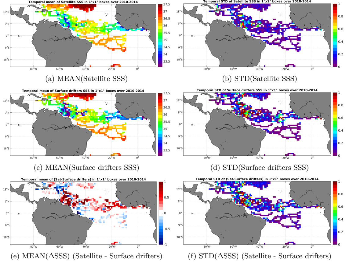
Figure 5: Temporal mean (left) and STD (right) of SSS from SMOS-L3-BEC-OA-V1-9DAYS-0.25DEG (top), Surface drifters (middle), and of \Delta\text{SSS} (Satellite - Surface drifters). Only match-up pairs are used to generate these maps.
