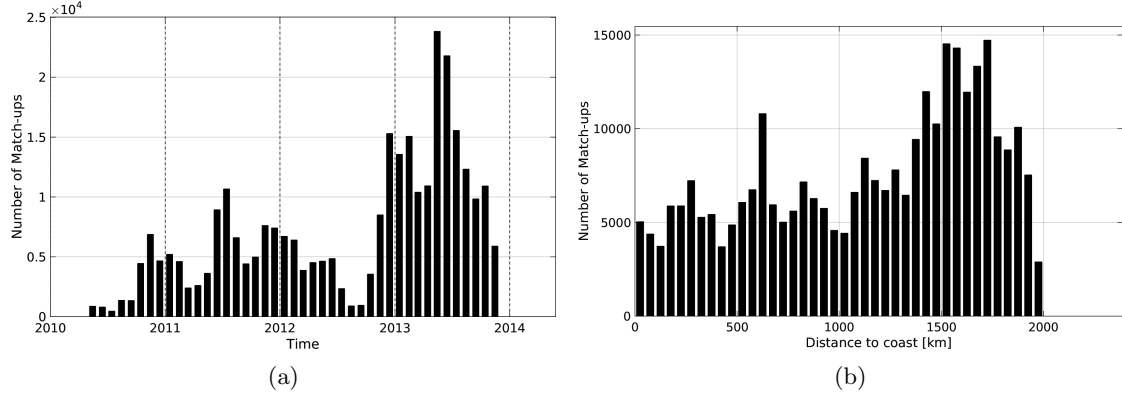
Figure 1: Number of match-ups between Surface drifters and SMOS-L3-BEC-OA-V1-9DAYS-0.25DEG SSS as a function of time (a) and as function of the distance to coast (b) over the Tropical Atlantic Ocean Pi-MEP region and for the full satellite product period.
