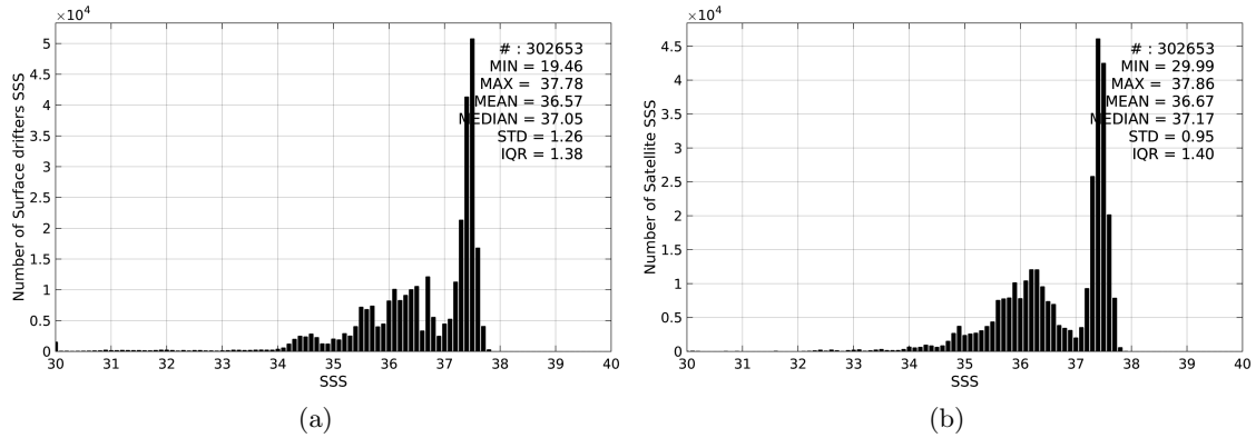
Figure 2: Histograms of SSS from Surface drifters (a) and SMOS-L3-BEC-OA-V1-9DAYS-0.25DEG (b) considering all match-up pairs per bins of 0.1 over the Tropical Atlantic Ocean Pi-MEP region and for the full satellite product period.
