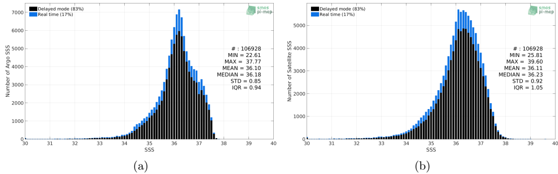
Figure 2: Histograms of SSS from Argo (a) and SMOS SSS L2-AVERAGED v700 (ESA) (b) considering all match-up pairs per bins of 0.1 over the Tropical Atlantic Ocean Pi-MEP region and for the full satellite product period.
