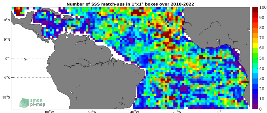
Figure 4: Number of SSS match-ups between Argo SSS and the SMOS SSS L2-AVERAGED v700 (ESA) SSS product for the Tropical Atlantic Ocean Pi-MEP region over 1^\circ \times 1^\circ boxes and for the full satellite product period.
