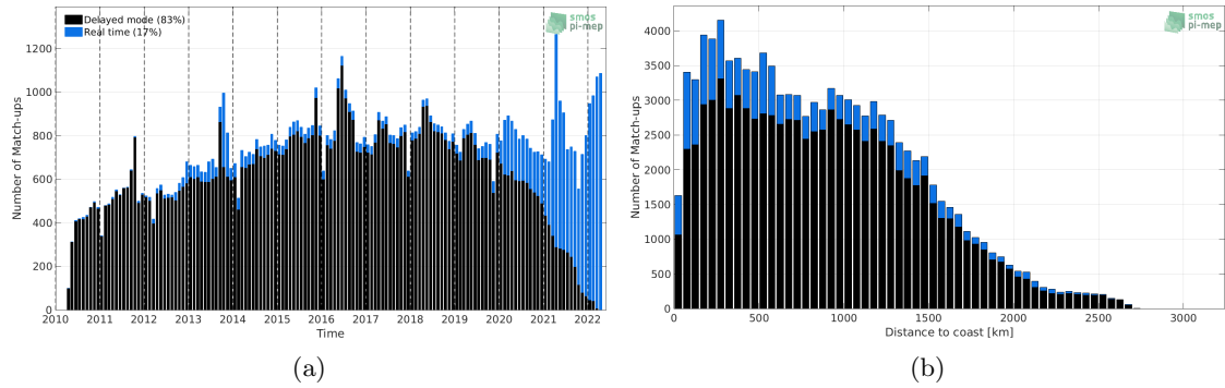
Figure 1: Number of match-ups between Argo and SMOS SSS L2-AVERAGED v700 (ESA) SSS as a function of time (a) and as function of the distance to coast (b) over the Tropical Atlantic Ocean Pi-MEP region and for the full satellite product period.
