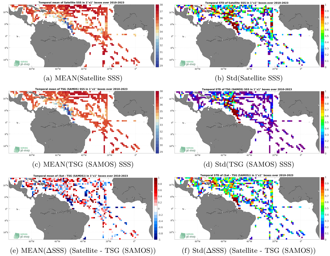
Figure 6: Temporal mean (left) and Std (right) of SSS from SMOS SSS L2 v700 (ESA) (top), TSG (SAMOS) (middle), and of \Delta SSS (Satellite - TSG (SAMOS)). Only match-up pairs are used to generate these maps.
