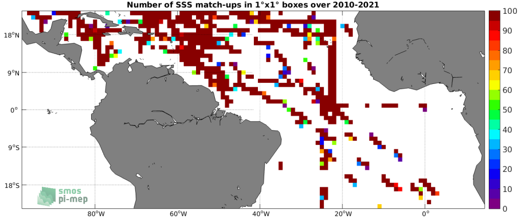
Figure 4: Number of SSS match-ups between TSG (SAMOS) SSS and the SMOS SSS L2 v700 (ESA) SSS product for the Tropical Atlantic Ocean Pi-MEP region over 1^\circ \times 1^\circ boxes and for the full satellite product period.
