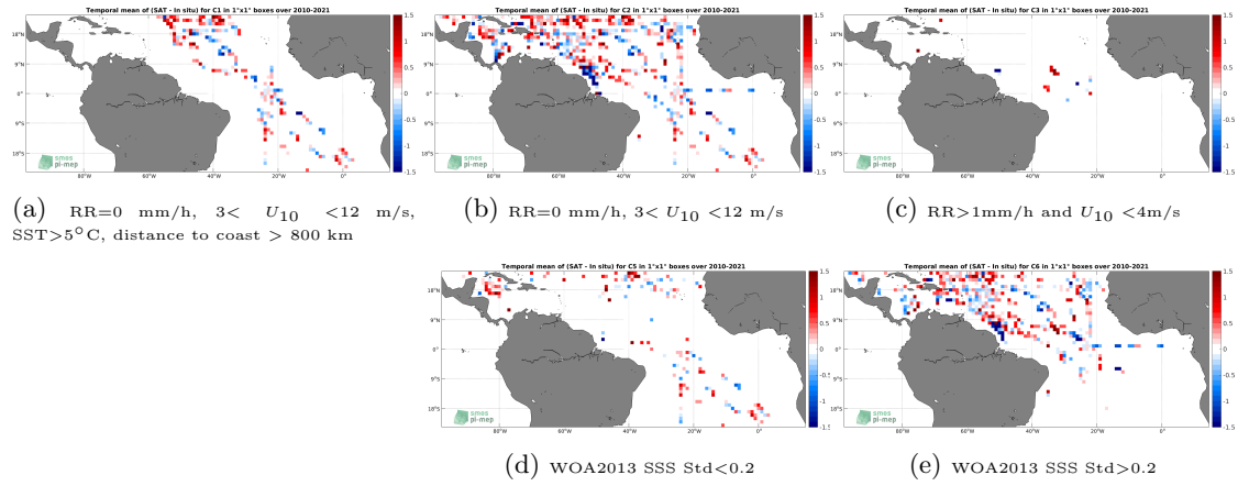
Figure 12: Temporal mean gridded over spatial boxes of size 1^\circ \times 1^\circ of \Delta SSS (SMOS SSS L2 v700 (ESA) - TSG (SAMOS)) for 5 different subdatasets corresponding to:RR=0 mm/h, 3 < U_{10} < 12 m/s, SST >5^\circ\text{C} , distance to coast > 800 km (a), RR=0 mm/h, 3 < U_{10} < 12 m/s (b), RR >1 mm/h and U_{10} < 4 m/s (c), WOA2013 SSS Std <0.2 (d), WOA2013 SSS Std >0.2 (e).
