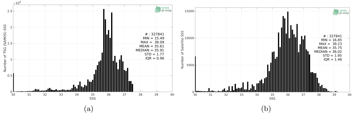
Figure 2: Histograms of SSS from TSG (SAMOS) (a) and SMOS SSS L2 v700 (ESA) (b) considering all match-up pairs per bins of 0.1 over the Tropical Atlantic Ocean Pi-MEP region and for the full satellite product period.
