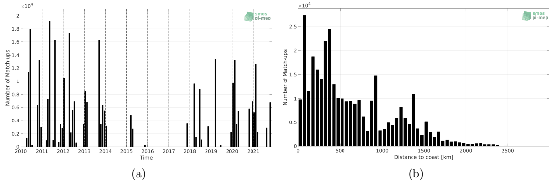
Figure 1: Number of match-ups between TSG (SAMOS) and SMOS SSS L2 v700 (ESA) SSS as a function of time (a) and as function of the distance to coast (b) over the Tropical Atlantic Ocean Pi-MEP region and for the full satellite product period.
