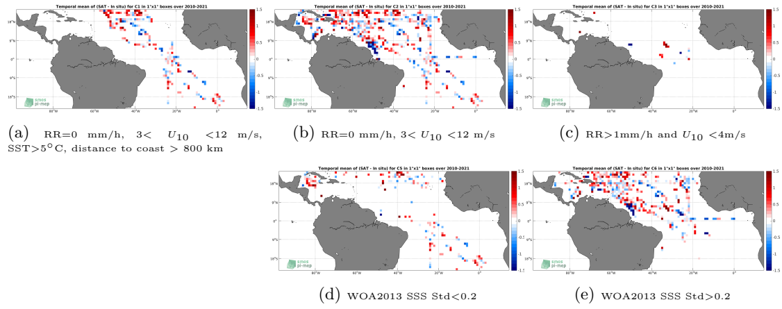
Figure 12: Temporal mean gridded over spatial boxes of size 1^\circ \times 1^\circ of \Delta SSS (SMOS SSS L2 v700 (ESA) - TSG (SAMOS)) for 5 different subdatasets corresponding to: RR=0 mm/h, 3 < U_{10} < 12 m/s, SST > 5^\circ C , distance to coast > 800 km (a), RR=0 mm/h, 3 < U_{10} < 12 m/s (b), RR > 1 mm/h and U_{10} < 4 m/s (c), WOA2013 SSS Std < 0.2 (d), WOA2013 SSS Std > 0.2 (e).
