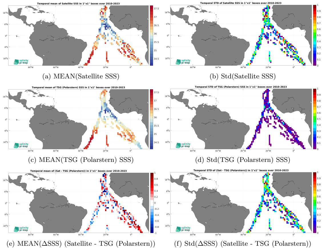
Figure 7: Temporal mean (left) and Std (right) of SSS from SMOS SSS L2 v700 (ESA) (top), TSG (Polarstern) (middle), and of \Delta SSS (Satellite - TSG (Polarstern)). Only match-up pairs are used to generate these maps.
