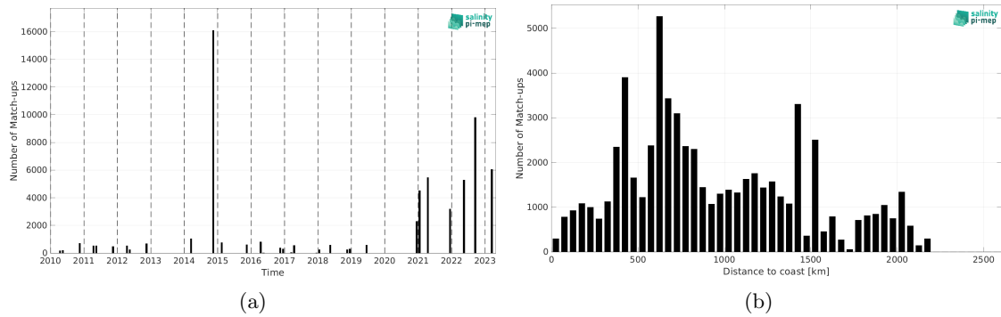
Figure 2: Number of match-ups between TSG (Polarstern) and SMOS SSS L2 v700 (ESA) SSS as a function of time (a) and as function of the distance to coast (b) over the Tropical Atlantic Ocean Pi-MEP region and for the full satellite product period.
