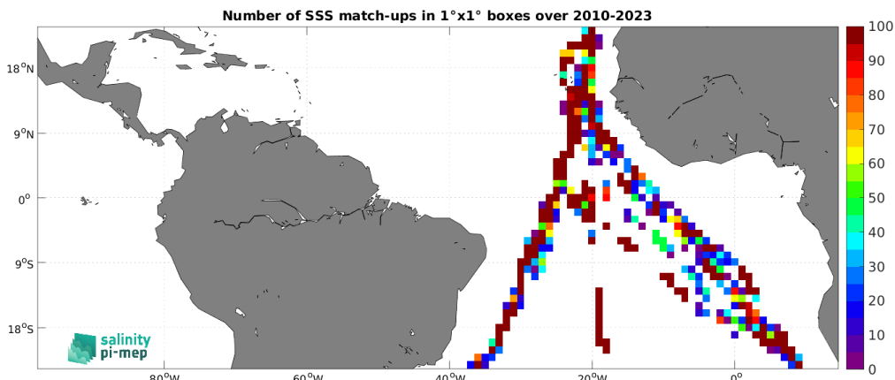
Figure 5: Number of SSS match-ups between TSG (Polarstern) SSS and the SMOS SSS L2 v700 (ESA) SSS product for the Tropical Atlantic Ocean Pi-MEP region over 1^\circ \times 1^\circ boxes and for the full satellite product period.
