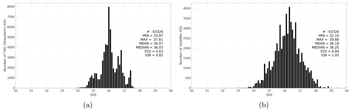
Figure 3: Histograms of SSS from TSG (Polarstern) (a) and SMOS SSS L2 v700 (ESA) (b) considering all match-up pairs per bins of 0.1 over the Tropical Atlantic Ocean Pi-MEP region and for the full satellite product period.
