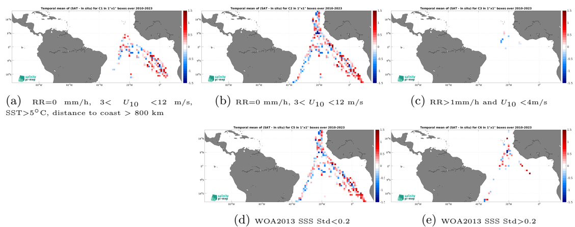
Figure 14: Temporal mean gridded over spatial boxes of size 1^\circ \times 1^\circ of \Delta\text{SSS} (SMOS SSS L2 v700 (ESA) - TSG (Polarstern)) for 5 different subdatasets corresponding to:RR=0 mm/h, 3 < U_{10} < 12 m/s, SST > 5°C, distance to coast > 800 km (a), RR=0 mm/h, 3 < U_{10} < 12 m/s (b), RR > 1mm/h and U_{10} < 4 m/s (c), WOA2013 SSS Std < 0.2 (d), WOA2013 SSS Std > 0.2 (e).
