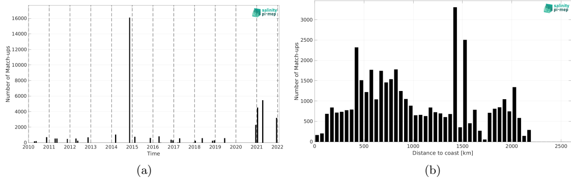
Figure 1: Number of match-ups between TSG (Polarstern) and SMOS SSS L2 v700 (ESA) SSS as a function of time (a) and as function of the distance to coast (b) over the Tropical Atlantic Ocean Pi-MEP region and for the full satellite product period.
