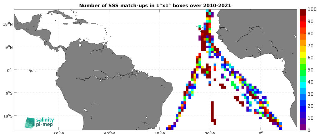
Figure 4: Number of SSS match-ups between TSG (Polarstern) SSS and the SMOS SSS L2 v700 (ESA) SSS product for the Tropical Atlantic Ocean Pi-MEP region over 1^\circ \times 1^\circ boxes and for the full satellite product period.
