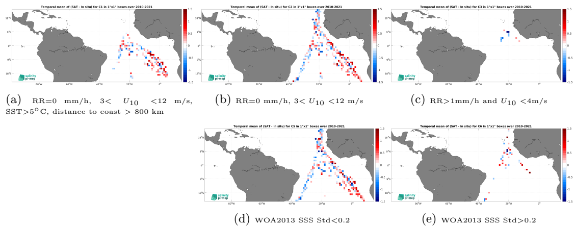
Figure 12: Temporal mean gridded over spatial boxes of size 1^\circ \times 1^\circ of \Delta\text{SSS} (SMOS SSS L2 v700 (ESA) - TSG (Polarstern)) for 5 different subdatasets corresponding to:RR=0 mm/h, 3 < U_{10} < 12 m/s, SST >5^\circ\text{C} , distance to coast > 800 km (a), RR=0 mm/h, 3 < U_{10} < 12 m/s (b), RR >1 mm/h and U_{10} < 4 m/s (c), WOA2013 SSS Std <0.2 (d), WOA2013 SSS Std >0.2 (e).
