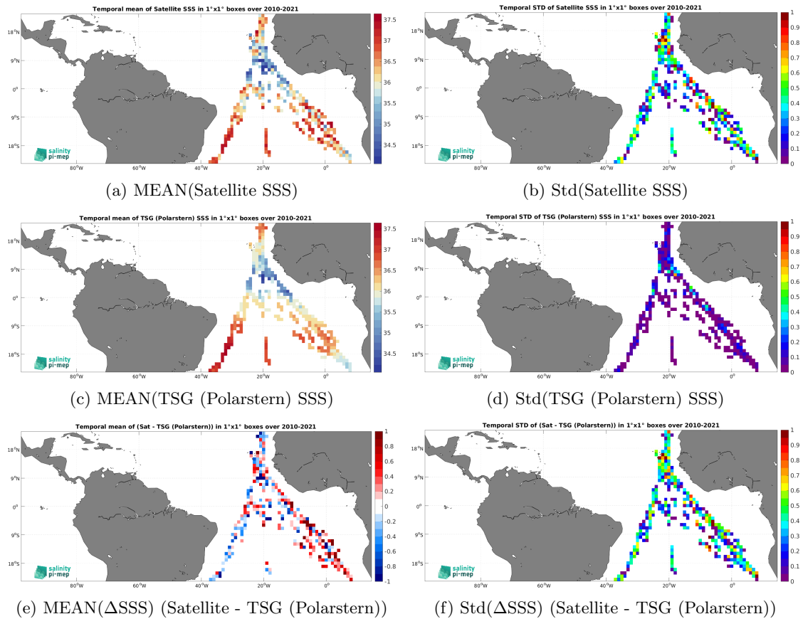
Figure 6: Temporal mean (left) and Std (right) of SSS from SMOS SSS L2 v700 (ESA) (top), TSG (Polarstern) (middle), and of \Delta SSS (Satellite - TSG (Polarstern)). Only match-up pairs are used to generate these maps.
