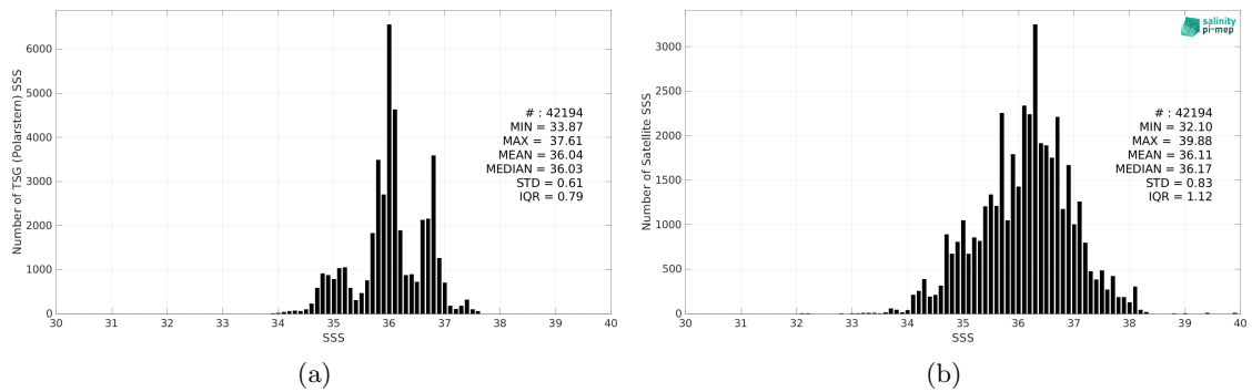
Figure 2: Histograms of SSS from TSG (Polarstern) (a) and SMOS SSS L2 v700 (ESA) (b) considering all match-up pairs per bins of 0.1 over the Tropical Atlantic Ocean Pi-MEP region and for the full satellite product period.
