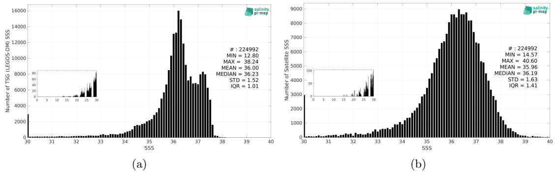
Figure 3: Histograms of SSS from TSG (LEGOS-DM) (a) and SMOS SSS L2 v700 (ESA) (b) considering all match-up pairs per bins of 0.1 over the Tropical Atlantic Ocean Pi-MEP region and for the full satellite product period.
