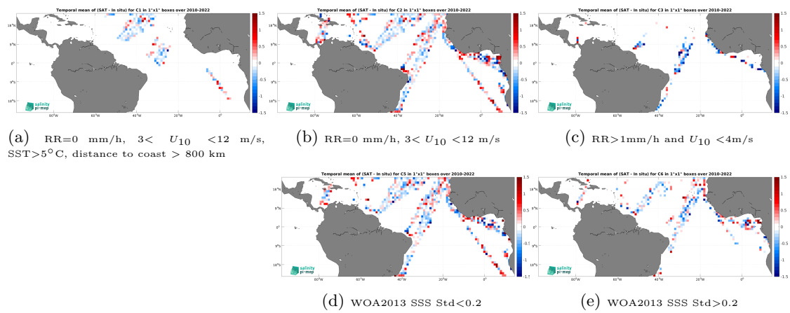
Figure 14: Temporal mean gridded over spatial boxes of size 1^\circ \times 1^\circ of \Delta SSS (SMOS SSS L2 v700 (ESA) - TSG (LEGOS-DM)) for 5 different subdatasets corresponding to: RR=0 mm/h, 3 < U_{10} < 12 m/s, SST > 5°C, distance to coast > 800 km (a), RR=0 mm/h, 3 < U_{10} < 12 m/s (b), RR > 1mm/h and U_{10} < 4 m/s (c), WOA2013 SSS Std < 0.2 (d), WOA2013 SSS Std > 0.2 (e).
