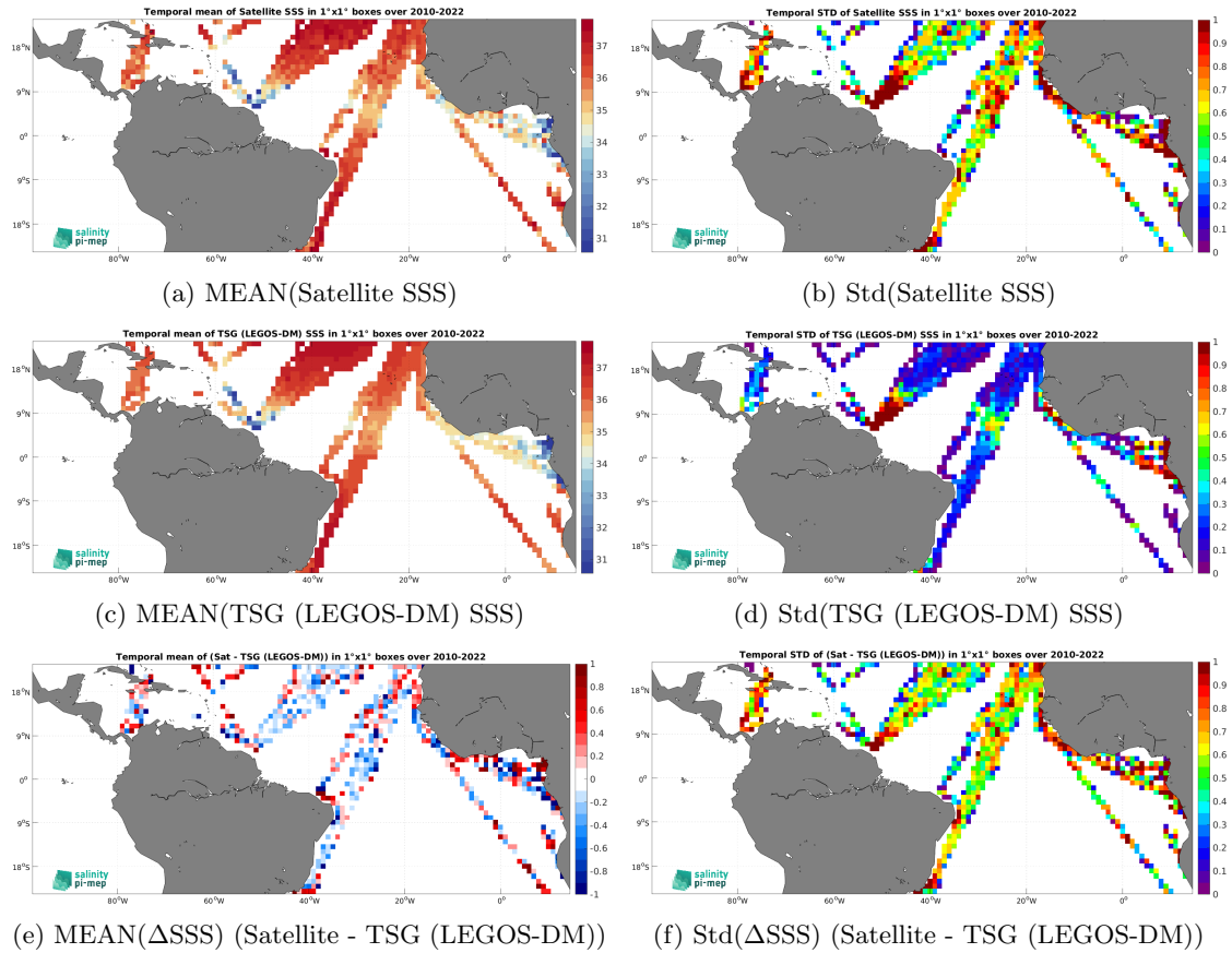
Figure 7: Temporal mean (left) and Std (right) of SSS from SMOS SSS L2 v700 (ESA) (top), TSG (LEGOS-DM) (middle), and of \Delta SSS (Satellite - TSG (LEGOS-DM)). Only match-up pairs are used to generate these maps.
