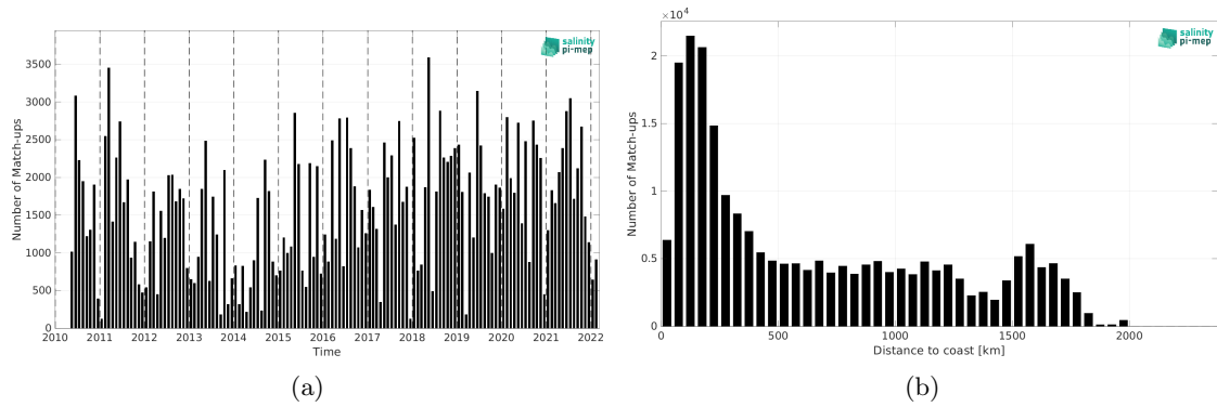
Figure 2: Number of match-ups between TSG (LEGOS-DM) and SMOS SSS L2 v700 (ESA) SSS as a function of time (a) and as function of the distance to coast (b) over the Tropical Atlantic Ocean Pi-MEP region and for the full satellite product period.
