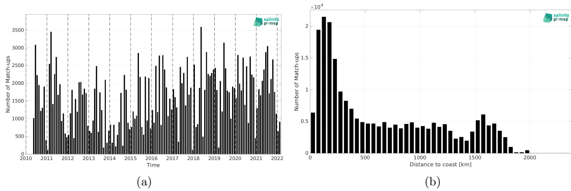
Figure 1: Number of match-ups between TSG (LEGOS-DM) and SMOS SSS L2 v700 (ESA) SSS as a function of time (a) and as function of the distance to coast (b) over the Tropical Atlantic Ocean Pi-MEP region and for the full satellite product period.
