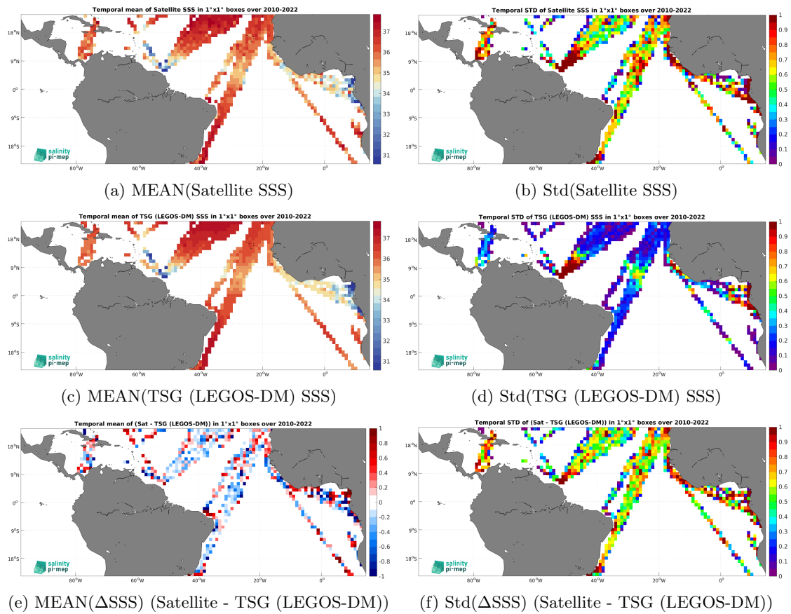
Figure 6: Temporal mean (left) and Std (right) of SSS from SMOS SSS L2 v700 (ESA) (top), TSG (LEGOS-DM) (middle), and of \Delta SSS (Satellite - TSG (LEGOS-DM)). Only match-up pairs are used to generate these maps.
