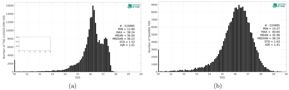
Figure 2: Histograms of SSS from TSG (LEGOS-DM) (a) and SMOS SSS L2 v700 (ESA) (b) considering all match-up pairs per bins of 0.1 over the Tropical Atlantic Ocean Pi-MEP region and for the full satellite product period.
