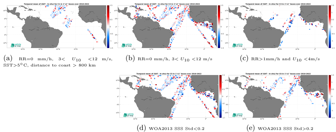
Figure 12: Temporal mean gridded over spatial boxes of size 1^\circ \times 1^\circ of \Delta\text{SSS} (SMOS SSS L2 v700 (ESA) - TSG (LEGOS-DM)) for 5 different subdatasets corresponding to:RR=0 mm/h, 3 < U_{10} < 12 m/s, SST >5^\circ\text{C} , distance to coast > 800 km (a), RR=0 mm/h, 3 < U_{10} < 12 m/s (b), RR >1 mm/h and U_{10} < 4 m/s (c), WOA2013 SSS Std <0.2 (d), WOA2013 SSS Std >0.2 (e).
