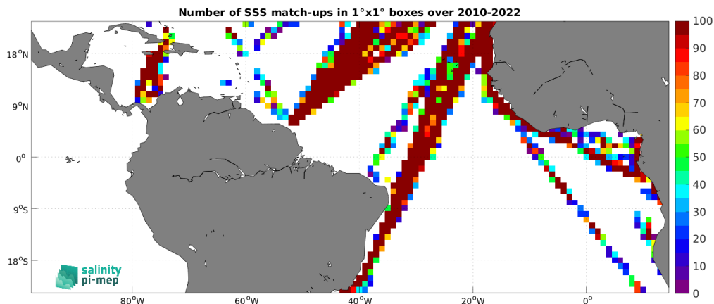
Figure 4: Number of SSS match-ups between TSG (LEGOS-DM) SSS and the SMOS SSS L2 v700 (ESA) SSS product for the Tropical Atlantic Ocean Pi-MEP region over 1^\circ \times 1^\circ boxes and for the full satellite product period.
