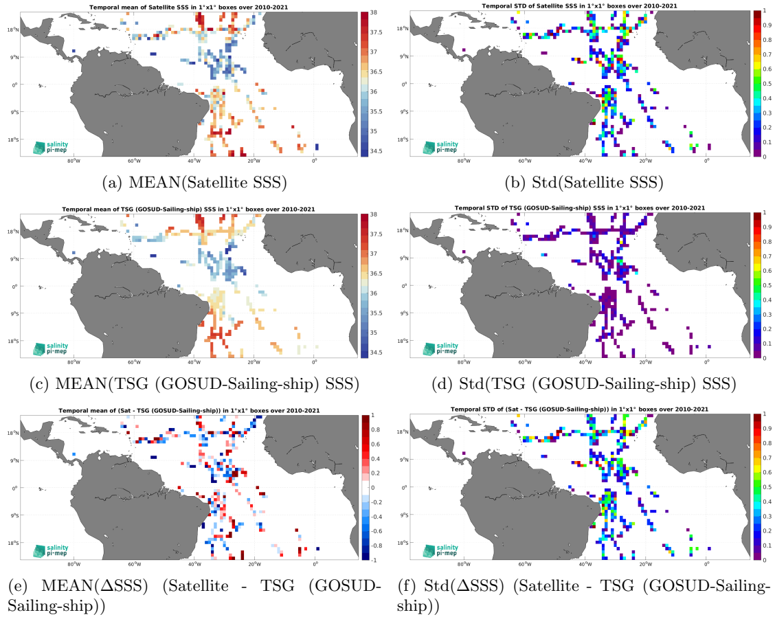
Figure 7: Temporal mean (left) and Std (right) of SSS from SMOS SSS L2 v700 (ESA) (top), TSG (GOSUD-Sailing-ship) (middle), and of \Delta SSS (Satellite - TSG (GOSUD-Sailing-ship)). Only match-up pairs are used to generate these maps.
