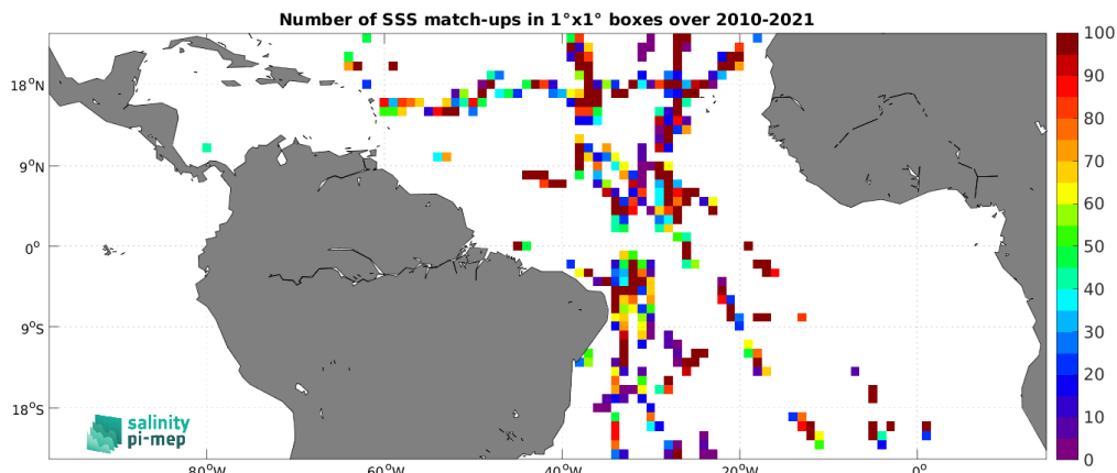
Figure 5: Number of SSS match-ups between TSG (GOSUD-Sailing-ship) SSS and the SMOS SSS L2 v700 (ESA) SSS product for the Tropical Atlantic Ocean Pi-MEP region over 1^\circ \times 1^\circ boxes and for the full satellite product period.
