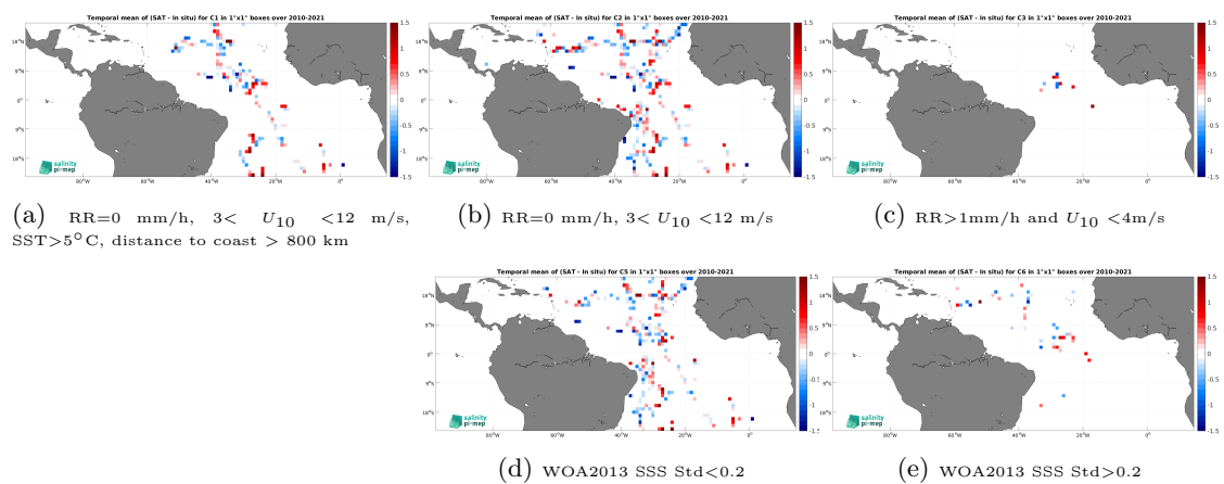
Figure 14: Temporal mean gridded over spatial boxes of size 1^\circ \times 1^\circ of \Delta\text{SSS} (SMOS SSS L2 v700 (ESA) - TSG (GOSUD-Sailing-ship)) for 5 different subdatasets corresponding to:RR=0 mm/h, 3 < U_{10} < 12 m/s, SST >5^\circ\text{C} , distance to coast > 800 km (a), RR=0 mm/h, 3 < U_{10} < 12 m/s (b), RR >1 mm/h and U_{10} < 4 m/s (c), WOA2013 SSS Std <0.2 (d), WOA2013 SSS Std >0.2 (e).
