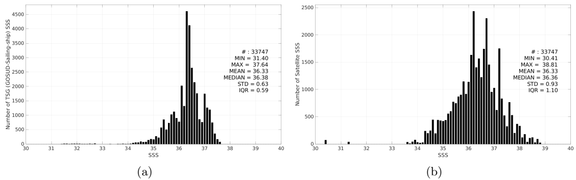
Figure 3: Histograms of SSS from TSG (GOSUD-Sailing-ship) (a) and SMOS SSS L2 v700 (ESA) (b) considering all match-up pairs per bins of 0.1 over the Tropical Atlantic Ocean Pi-MEP region and for the full satellite product period.
