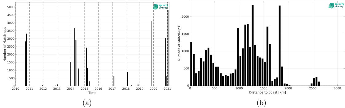
Figure 2: Number of match-ups between TSG (GOSUD-Sailing-ship) and SMOS SSS L2 v700 (ESA) SSS as a function of time (a) and as function of the distance to coast (b) over the Tropical Atlantic Ocean Pi-MEP region and for the full satellite product period.
