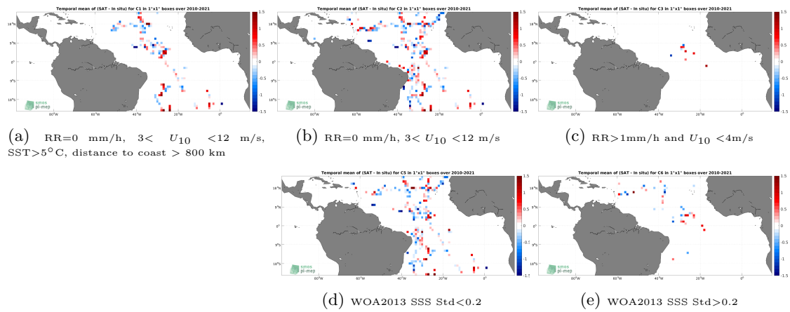
Figure 12: Temporal mean gridded over spatial boxes of size 1^\circ \times 1^\circ of \Delta SSS (SMOS SSS L2 v700 (ESA) - TSG (GOSUD-Sailing-ship)) for 5 different subdatasets corresponding to:RR=0 mm/h, 3 < U_{10} < 12 m/s, SST>5°C, distance to coast > 800 km (a), RR=0 mm/h, 3 < U_{10} < 12 m/s (b), RR>1mm/h and U_{10} < 4 m/s (c), WOA2013 SSS Std<0.2 (d), WOA2013 SSS Std>0.2 (e).
