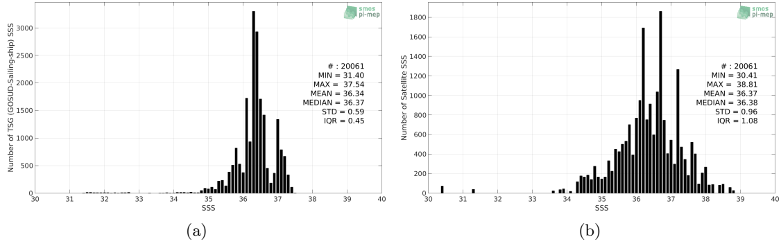
Figure 2: Histograms of SSS from TSG (GOSUD-Sailing-ship) (a) and SMOS SSS L2 v700 (ESA) (b) considering all match-up pairs per bins of 0.1 over the Tropical Atlantic Ocean Pi-MEP region and for the full satellite product period.
