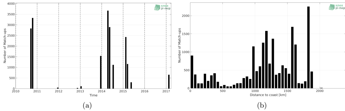
Figure 1: Number of match-ups between TSG (GOSUD-Sailing-ship) and SMOS SSS L2 v700 (ESA) SSS as a function of time (a) and as function of the distance to coast (b) over the Tropical Atlantic Ocean Pi-MEP region and for the full satellite product period.
