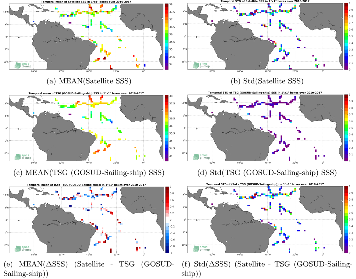
Figure 6: Temporal mean (left) and Std (right) of SSS from SMOS SSS L2 v700 (ESA) (top), TSG (GOSUD-Sailing-ship) (middle), and of \Delta\text{SSS} (Satellite - TSG (GOSUD-Sailing-ship)). Only match-up pairs are used to generate these maps.
