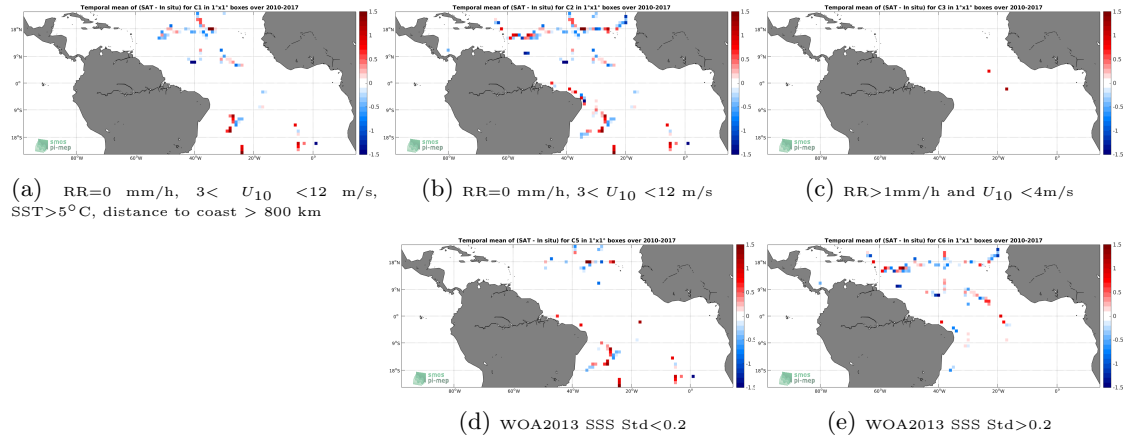
Figure 12: Temporal mean gridded over spatial boxes of size 1^\circ \times 1^\circ of \Delta SSS (SMOS SSS L2 v700 (ESA) - TSG (GOSUD-Sailing-ship)) for 5 different subdatasets corresponding to: RR=0 mm/h, 3 < U_{10} < 12 m/s, SST > 5^\circ C , distance to coast > 800 km (a), RR=0 mm/h, 3 < U_{10} < 12 m/s (b), RR > 1 mm/h and U_{10} < 4 m/s (c), WOA2013 SSS Std < 0.2 (d), WOA2013 SSS Std > 0.2 (e).
