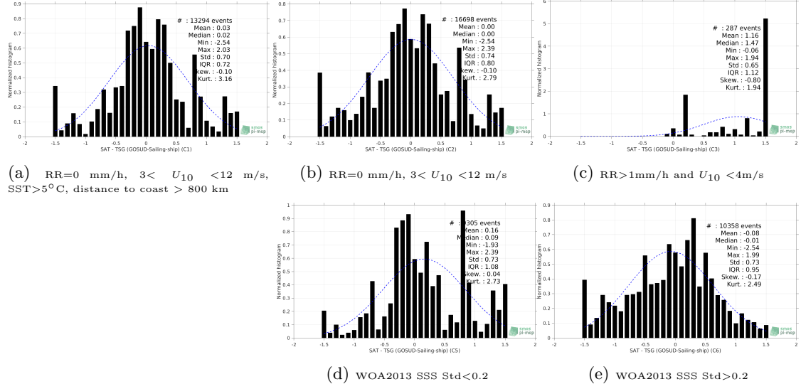
Figure 13: Normalized histogram of \Delta SSS (SMOS SSS L2 v700 (ESA) - TSG (GOSUD-Sailing-ship)) for 5 different subdatasets corresponding to: RR=0 mm/h, 3 < U_{10} < 12 m/s, SST>5°C, distance to coast > 800 km (a), RR=0 mm/h, 3 < U_{10} < 12 m/s (b), RR>1mm/h and U_{10} < 4 m/s (c), WOA2013 SSS Std<0.2 (d), WOA2013 SSS Std>0.2 (e).
