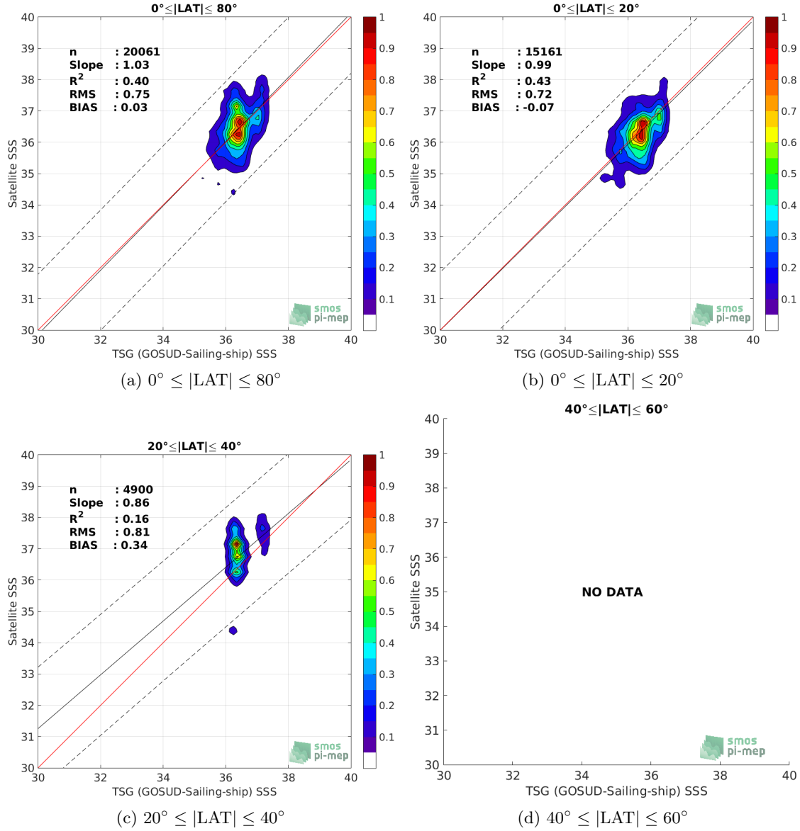
Figure 9: Contour maps of the concentration of SMOS SSS L2 v700 (ESA) SSS (y-axis) versus TSG (GOSUD-Sailing-ship) SSS (x-axis) at match-up pairs for different latitude bands. For each plot, the red line shows x=y . The black thin and dashed lines indicate a linear fit through the data cloud and the \pm 95\% confidence levels, respectively. The number match-up pairs n , the slope and R^2 coefficient of the linear fit, the root mean square (RMS) and the mean bias between satellite and in situ data are indicated for each latitude band in each plots.
