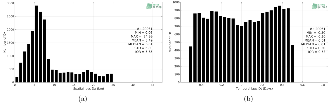
Figure 5: Histograms of the spatial (a) and temporal (b) lags between the location/time of the TSG (GOSUD-Sailing-ship) measurement and the date of the corresponding SMOS SSS L2 v700 (ESA) SSS pixel.
