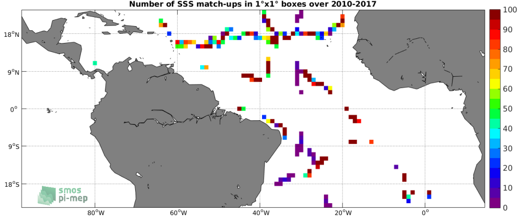
Figure 4: Number of SSS match-ups between TSG (GOSUD-Sailing-ship) SSS and the SMOS SSS L2 v700 (ESA) SSS product for the Tropical Atlantic Ocean Pi-MEP region over 1^\circ \times 1^\circ boxes and for the full satellite product period.
