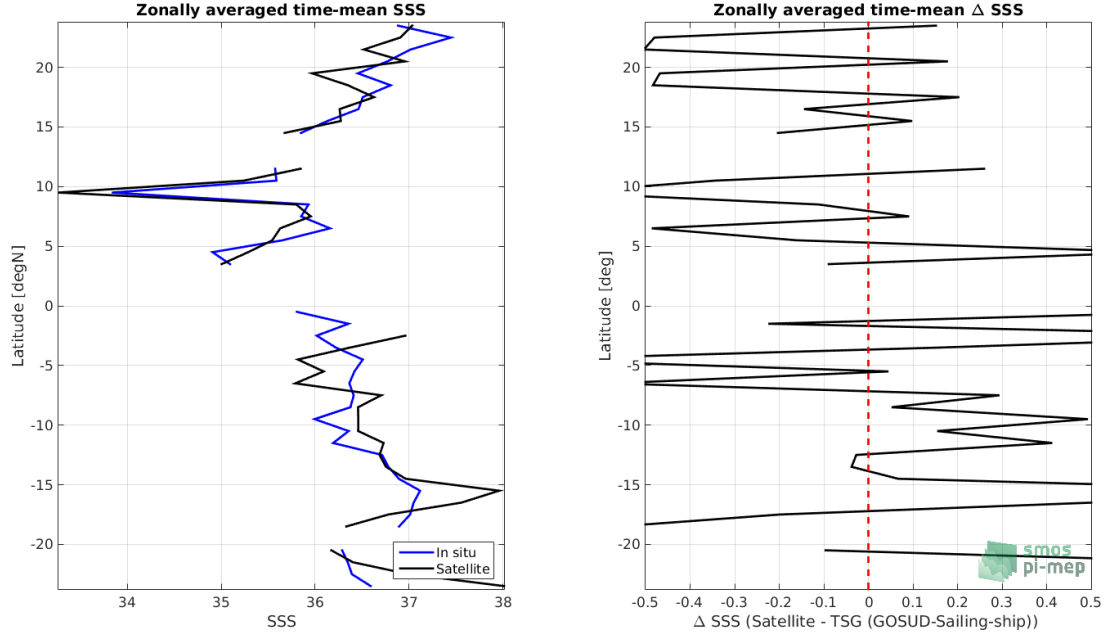
Figure 8: Left panel: Zonal mean SSS from SMOS SSS L2 v700 (ESA) satellite product (black) and from TSG (GOSUD-Sailing-ship) (blue). Right panel: Zonal mean of \Delta SSS (Satellite - TSG (GOSUD-Sailing-ship)) for all the collected Pi-MEP match-up pairs estimated over the full satellite product period.
