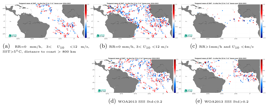
Figure 14: Temporal mean gridded over spatial boxes of size 1^\circ \times 1^\circ of \Delta SSS (SMOS SSS L2 v700 (ESA) - TSG (GOSUD-Research-vessel)) for 5 different subdatasets corresponding to:RR=0 mm/h, 3 < U_{10} < 12 m/s, SST>5°C, distance to coast > 800 km (a), RR=0 mm/h, 3 < U_{10} < 12 m/s (b), RR>1mm/h and U_{10} < 4 m/s (c), WOA2013 SSS Std<0.2 (d), WOA2013 SSS Std>0.2 (e).
