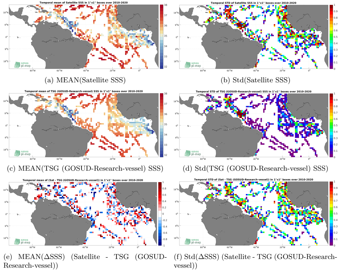
Figure 6: Temporal mean (left) and Std (right) of SSS from SMOS SSS L2 v700 (ESA) (top), TSG (GOSUD-Research-vessel) (middle), and of \Delta SSS (Satellite - TSG (GOSUD-Research-vessel)). Only match-up pairs are used to generate these maps.
