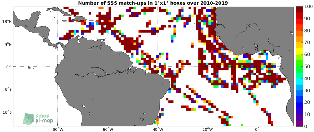
Figure 4: Number of SSS match-ups between TSG (GOSUD-Research-vessel) SSS and the SMOS SSS L2 v700 (ESA) SSS product for the Tropical Atlantic Ocean Pi-MEP region over 1^\circ \times 1^\circ boxes and for the full satellite product period.
