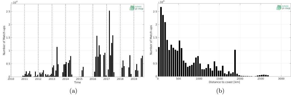
Figure 1: Number of match-ups between TSG (GOSUD-Research-vessel) and SMOS SSS L2 v700 (ESA) SSS as a function of time (a) and as function of the distance to coast (b) over the Tropical Atlantic Ocean Pi-MEP region and for the full satellite product period.
