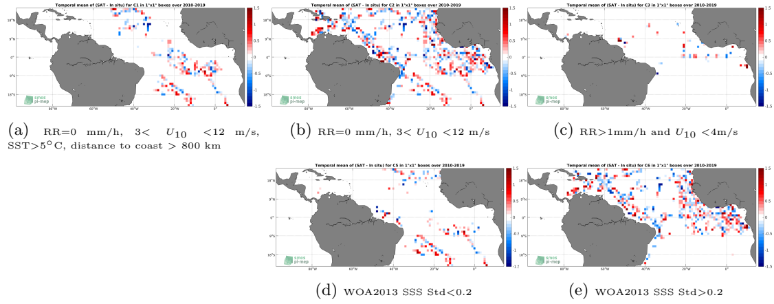
Figure 12: Temporal mean gridded over spatial boxes of size 1^\circ \times 1^\circ of \Delta SSS (SMOS SSS L2 v700 (ESA) - TSG (GOSUD-Research-vessel)) for 5 different subdatasets corresponding to: RR=0 mm/h, 3 < U_{10} < 12 m/s, SST >5^\circ\text{C} , distance to coast > 800 km (a), RR=0 mm/h, 3 < U_{10} < 12 m/s (b), RR >1 mm/h and U_{10} < 4 m/s (c), WOA2013 SSS Std <0.2 (d), WOA2013 SSS Std >0.2 (e).
