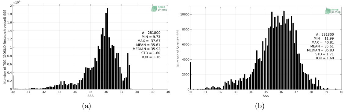
Figure 2: Histograms of SSS from TSG (GOSUD-Research-vessel) (a) and SMOS SSS L2 v700 (ESA) (b) considering all match-up pairs per bins of 0.1 over the Tropical Atlantic Ocean Pi-MEP region and for the full satellite product period.
