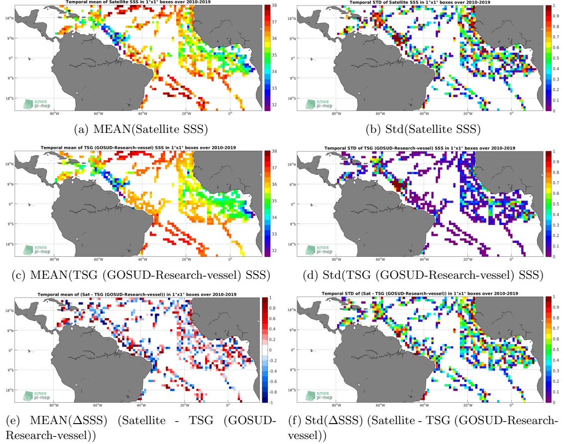
Figure 6: Temporal mean (left) and Std (right) of SSS from SMOS SSS L2 v700 (ESA) (top), TSG (GOSUD-Research-vessel) (middle), and of \Delta\text{SSS} (Satellite - TSG (GOSUD-Research-vessel)). Only match-up pairs are used to generate these maps.
