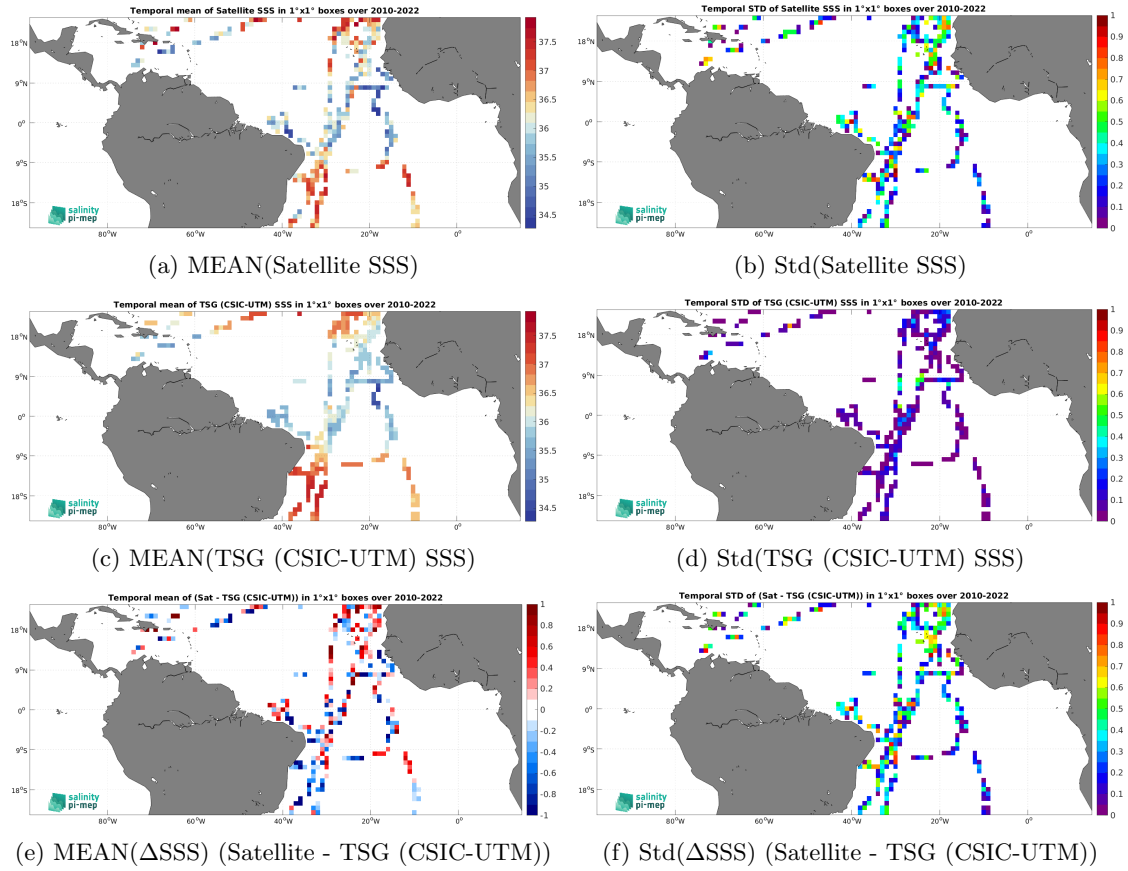
Figure 6: Temporal mean (left) and Std (right) of SSS from SMOS SSS L2 v700 (ESA) (top), TSG (CSIC-UTM) (middle), and of \Delta SSS (Satellite - TSG (CSIC-UTM)). Only match-up pairs are used to generate these maps.
