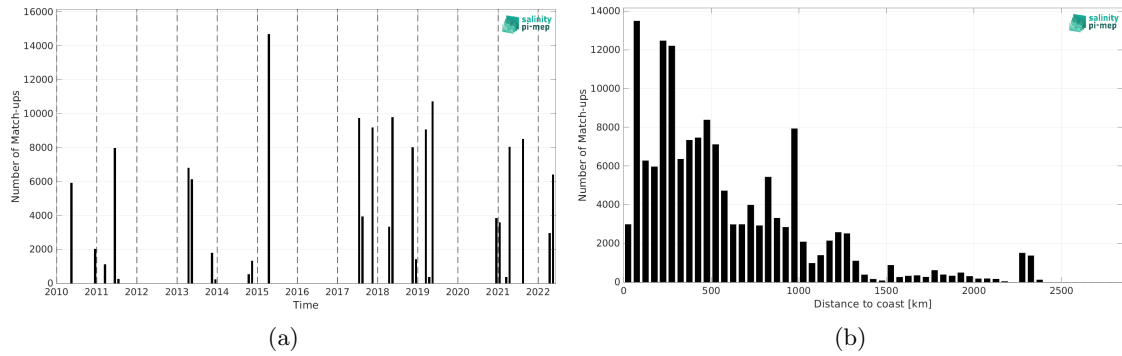
Figure 1: Number of match-ups between TSG (CSIC-UTM) and SMOS SSS L2 v700 (ESA) SSS as a function of time (a) and as function of the distance to the coast (b) over the Tropical Atlantic Ocean Pi-MEP region and for the full satellite product period.
