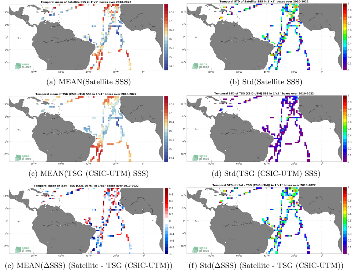
Figure 6: Temporal mean (left) and Std (right) of SSS from SMOS SSS L2 v700 (ESA) (top), TSG (CSIC-UTM) (middle), and of \Delta\text{SSS} (Satellite - TSG (CSIC-UTM)). Only match-up pairs are used to generate these maps.
