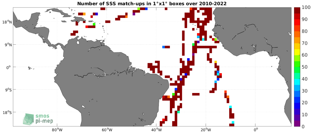
Figure 4: Number of SSS match-ups between TSG (CSIC-UTM) SSS and the SMOS SSS L2 v700 (ESA) SSS product for the Tropical Atlantic Ocean Pi-MEP region over 1^\circ \times 1^\circ boxes and for the full satellite product period.
