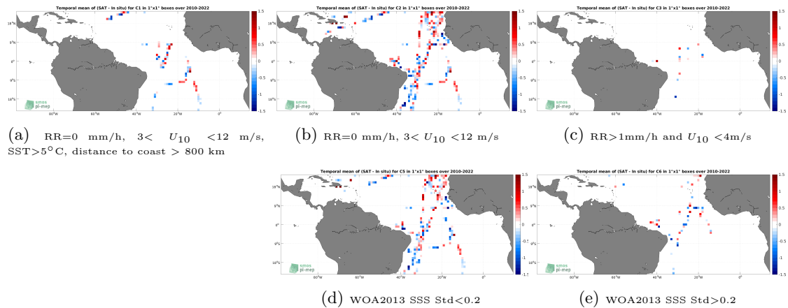
Figure 12: Temporal mean gridded over spatial boxes of size 1^\circ \times 1^\circ of \Delta SSS (SMOS SSS L2 v700 (ESA) - TSG (CSIC-UTM)) for 5 different subdatasets corresponding to:RR=0 mm/h, 3 < U_{10} < 12 m/s, SST >5^\circ\text{C} , distance to coast > 800 km (a), RR=0 mm/h, 3 < U_{10} < 12 m/s (b), RR >1 mm/h and U_{10} < 4 m/s (c), WOA2013 SSS Std <0.2 (d), WOA2013 SSS Std >0.2 (e).
