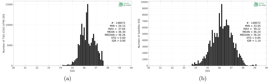
Figure 2: Histograms of SSS from TSG (CSIC-UTM) (a) and SMOS SSS L2 v700 (ESA) (b) considering all match-up pairs per bins of 0.1 over the Tropical Atlantic Ocean Pi-MEP region and for the full satellite product period.
