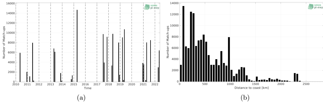
Figure 1: Number of match-ups between TSG (CSIC-UTM) and SMOS SSS L2 v700 (ESA) SSS as a function of time (a) and as function of the distance to coast (b) over the Tropical Atlantic Ocean Pi-MEP region and for the full satellite product period.
