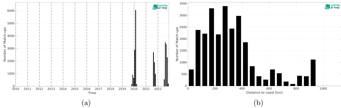
Figure 2: Number of match-ups between Saildrone and SMOS SSS L2 v700 (ESA) SSS as a function of time (a) and as function of the distance to coast (b) over the Tropical Atlantic Ocean Pi-MEP region and for the full satellite product period.
