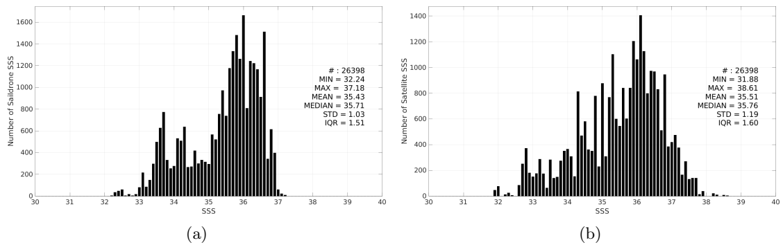
Figure 3: Histograms of SSS from Saildrone (a) and SMOS SSS L2 v700 (ESA) (b) considering all match-up pairs per bins of 0.1 over the Tropical Atlantic Ocean Pi-MEP region and for the full satellite product period.
