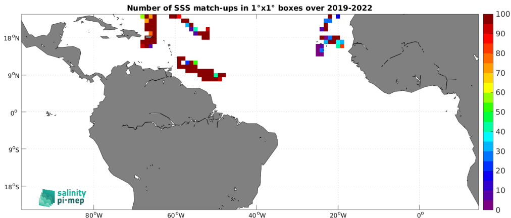
Figure 5: Number of SSS match-ups between Saildrone SSS and the SMOS SSS L2 v700 (ESA) SSS product for the Tropical Atlantic Ocean Pi-MEP region over 1^\circ \times 1^\circ boxes and for the full satellite product period.
