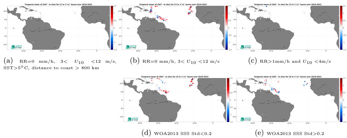
Figure 14: Temporal mean gridded over spatial boxes of size 1^\circ \times 1^\circ of \Delta\text{SSS} (SMOS SSS L2 v700 (ESA) - Sailability) for 5 different subdatasets corresponding to:RR=0 mm/h, 3 < U_{10} < 12 m/s, SST >5^\circ\text{C} , distance to coast > 800 km (a), RR=0 mm/h, 3 < U_{10} < 12 m/s (b), RR >1 mm/h and U_{10} < 4 m/s (c), WOA2013 SSS Std <0.2 (d), WOA2013 SSS Std >0.2 (e).
