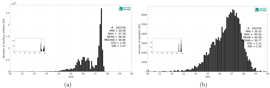
Figure 3: Histograms of SSS from Surface drifters (a) and SMOS SSS L2 v700 (ESA) (b) considering all match-up pairs per bins of 0.1 over the Tropical Atlantic Ocean Pi-MEP region and for the full satellite product period.
