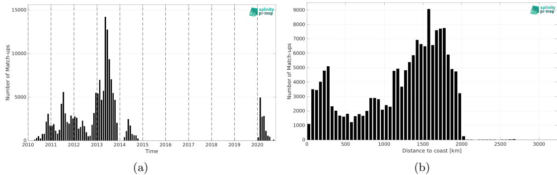
Figure 2: Number of match-ups between Surface drifters and SMOS SSS L2 v700 (ESA) SSS as a function of time (a) and as function of the distance to coast (b) over the Tropical Atlantic Ocean Pi-MEP region and for the full satellite product period.
