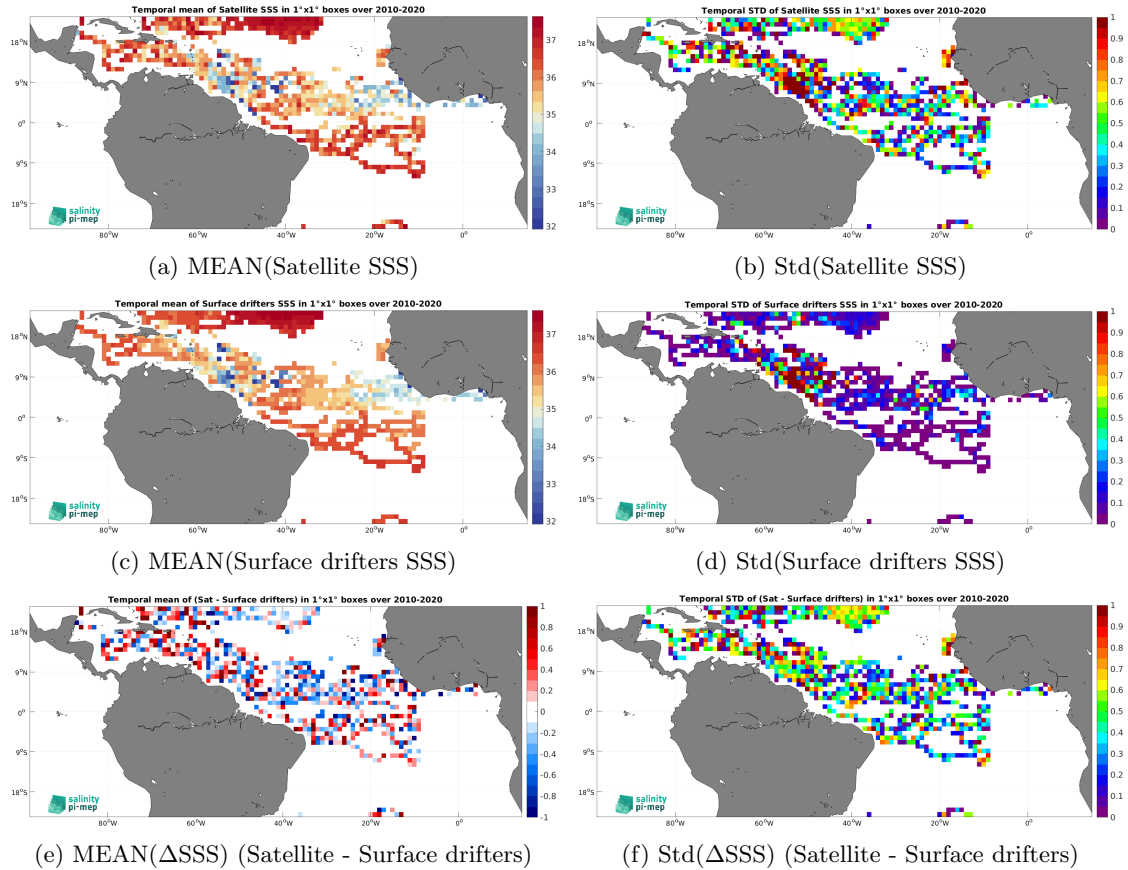
Figure 6: Temporal mean (left) and Std (right) of SSS from SMOS SSS L2 v700 (ESA) (top), Surface drifters (middle), and of \Delta SSS (Satellite - Surface drifters). Only match-up pairs are used to generate these maps.
