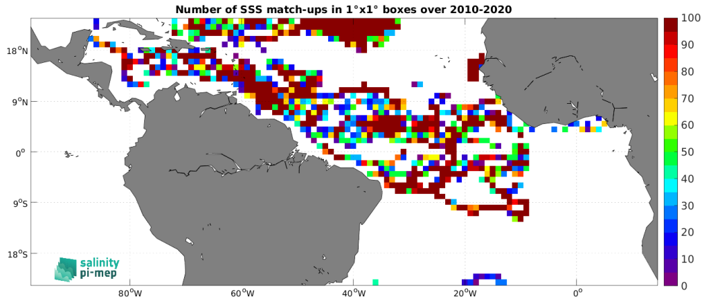
Figure 3: Number of SSS match-ups between Surface drifters SSS and the SMOS SSS L2 v700 (ESA) SSS product for the Tropical Atlantic Ocean Pi-MEP region over 1^{\circ} \times 1^{\circ} boxes and for the full satellite product period.
