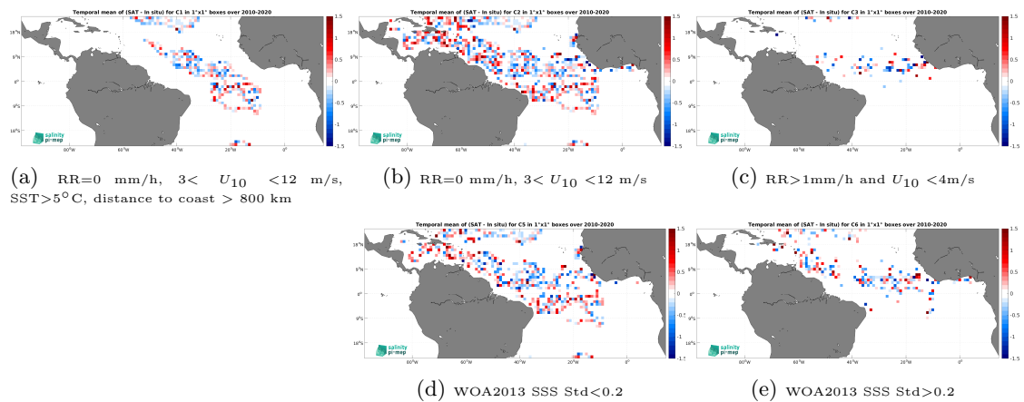
Figure 11: Temporal mean gridded over spatial boxes of size 1^\circ \times 1^\circ of \Delta\text{SSS} (SMOS SSS L2 v700 (ESA) - Surface drifters) for 5 different subdatasets corresponding to:RR=0 mm/h, 3 < U_{10} < 12 m/s, SST >5^\circ\text{C} , distance to coast > 800 km (a), RR=0 mm/h, 3 < U_{10} < 12 m/s (b), RR >1 mm/h and U_{10} < 4 m/s (c), WOA2013 SSS Std <0.2 (d), WOA2013 SSS Std >0.2 (e).
