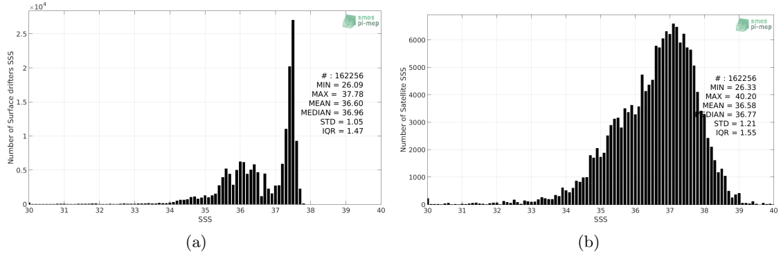
Figure 2: Histograms of SSS from Surface drifters (a) and SMOS SSS L2 v700 (ESA) (b) considering all match-up pairs per bins of 0.1 over the Tropical Atlantic Ocean Pi-MEP region and for the full satellite product period.
