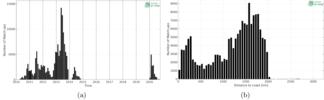
Figure 1: Number of match-ups between Surface drifters and SMOS SSS L2 v700 (ESA) SSS as a function of time (a) and as function of the distance to coast (b) over the Tropical Atlantic Ocean Pi-MEP region and for the full satellite product period.
