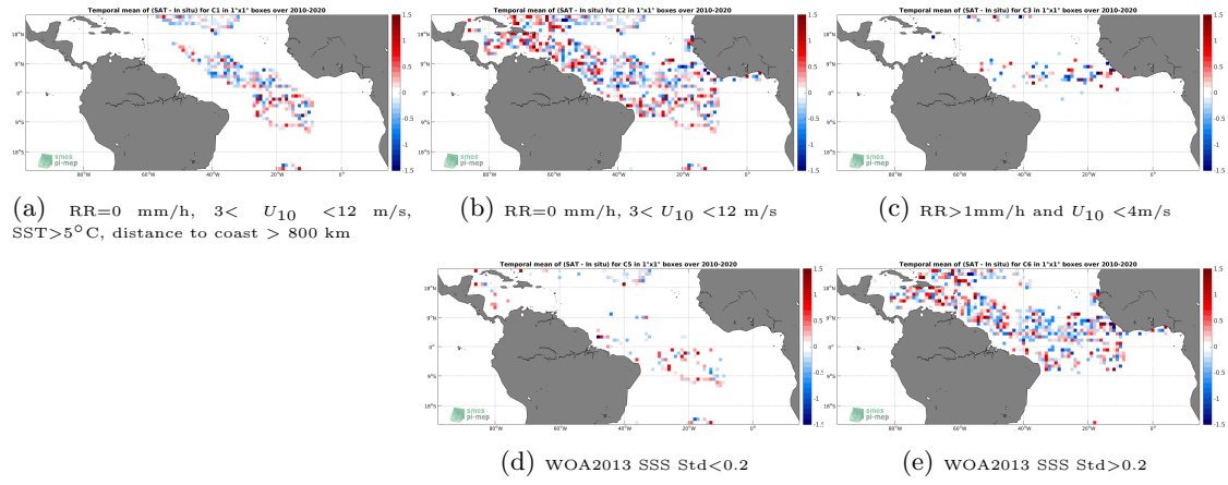
Figure 11: Temporal mean gridded over spatial boxes of size 1^\circ \times 1^\circ of \Delta SSS (SMOS SSS L2 v700 (ESA) - Surface drifters) for 5 different subdatasets corresponding to:RR=0 mm/h, 3 < U_{10} < 12 m/s, SST >5^\circ\text{C} , distance to coast > 800 km (a), RR=0 mm/h, 3 < U_{10} < 12 m/s (b), RR >1 mm/h and U_{10} < 4 m/s (c), WOA2013 SSS Std <0.2 (d), WOA2013 SSS Std >0.2 (e).
