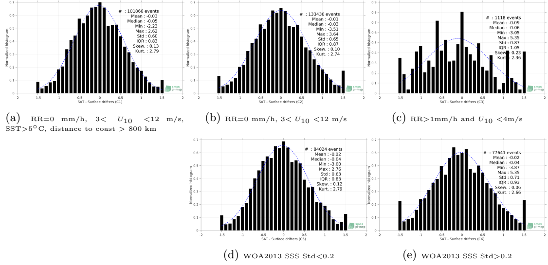
Figure 12: Normalized histogram of \Delta SSS (SMOS SSS L2 v700 (ESA) - Surface drifters) for 5 different subdatasets corresponding to: RR=0 mm/h, 3 < U_{10} < 12 m/s, SST>5°C, distance to coast > 800 km (a), RR=0 mm/h, 3 < U_{10} < 12 m/s (b), RR>1mm/h and U_{10} < 4 m/s (c), WOA2013 SSS Std<0.2 (d), WOA2013 SSS Std>0.2 (e).
