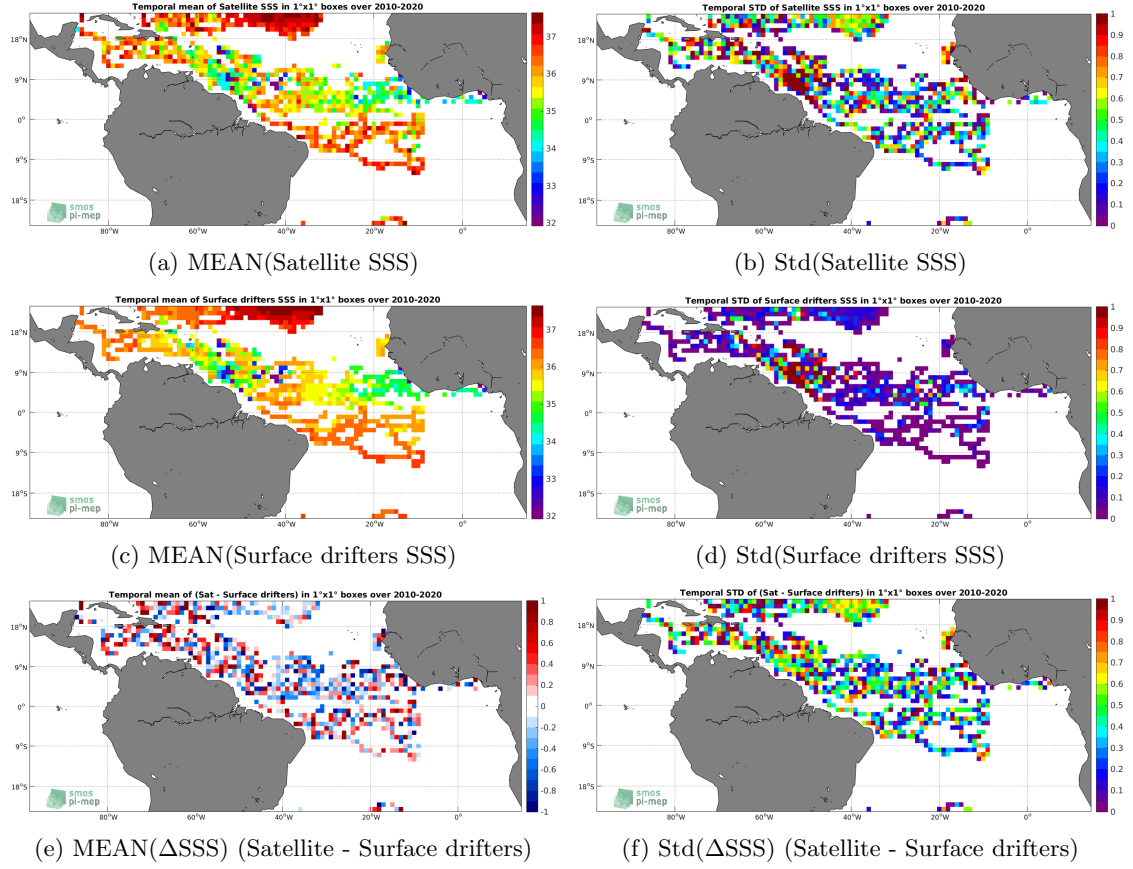
Figure 5: Temporal mean (left) and Std (right) of SSS from SMOS SSS L2 v700 (ESA) (top), Surface drifters (middle), and of \Delta SSS (Satellite - Surface drifters). Only match-up pairs are used to generate these maps.
