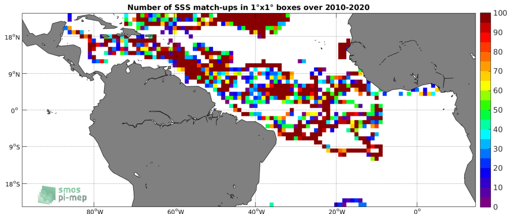
Figure 3: Number of SSS match-ups between Surface drifters SSS and the SMOS SSS L2 v700 (ESA) SSS product for the Tropical Atlantic Ocean Pi-MEP region over 1^\circ \times 1^\circ boxes and for the full satellite product period.
