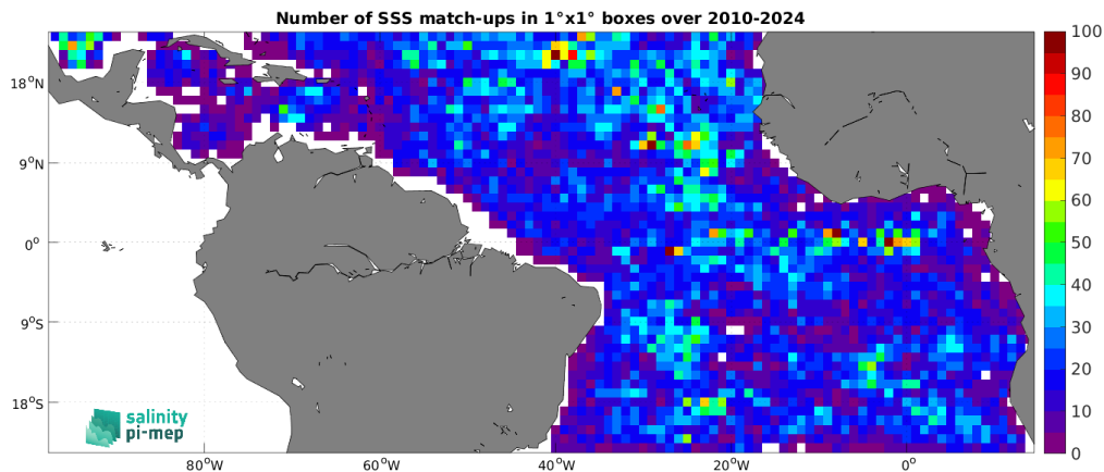
Figure 5: Number of SSS match-ups between Argo SSS and the SMOS SSS L2 v700 (ESA) SSS product for the Tropical Atlantic Ocean Pi-MEP region over 1^\circ \times 1^\circ boxes and for the full satellite product period.
