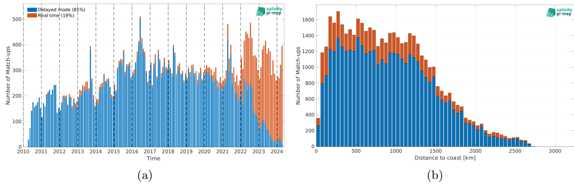
Figure 2: Number of match-ups between Argo and SMOS SSS L2 v700 (ESA) SSS as a function of time (a) and as function of the distance to coast (b) over the Tropical Atlantic Ocean Pi-MEP region and for the full satellite product period.
