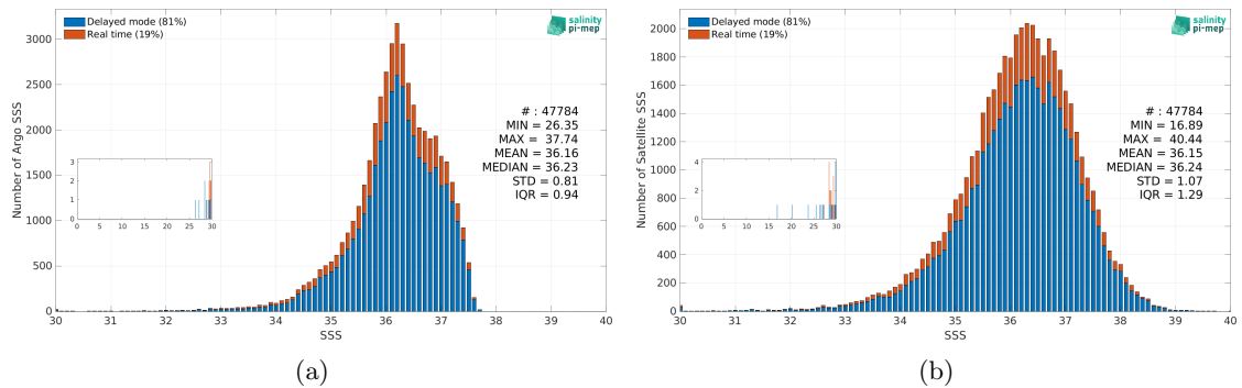
Figure 3: Histograms of SSS from Argo (a) and SMOS SSS L2 v700 (ESA) (b) considering all match-up pairs per bins of 0.1 over the Tropical Atlantic Ocean Pi-MEP region and for the full satellite product period.
