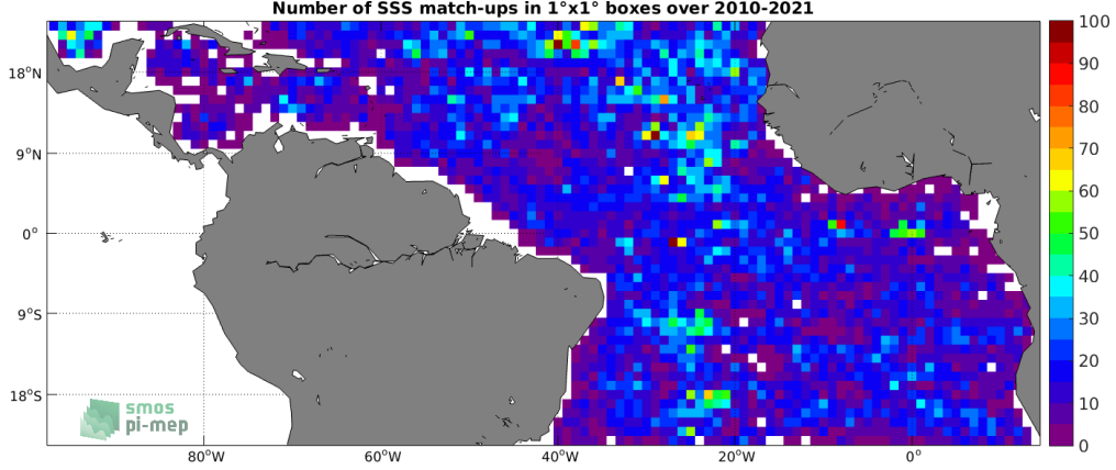
Figure 4: Number of SSS match-ups between Argo SSS and the SMOS SSS L2 v700 (ESA) SSS product for the Tropical Atlantic Ocean Pi-MEP region over 1^\circ \times 1^\circ boxes and for the full satellite product period.
