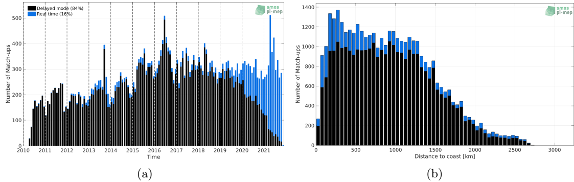
Figure 1: Number of match-ups between Argo and SMOS SSS L2 v700 (ESA) SSS as a function of time (a) and as function of the distance to coast (b) over the Tropical Atlantic Ocean Pi-MEP region and for the full satellite product period.
