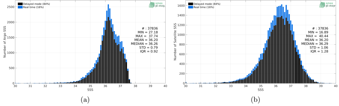
Figure 2: Histograms of SSS from Argo (a) and SMOS SSS L2 v700 (ESA) (b) considering all match-up pairs per bins of 0.1 over the Tropical Atlantic Ocean Pi-MEP region and for the full satellite product period.
