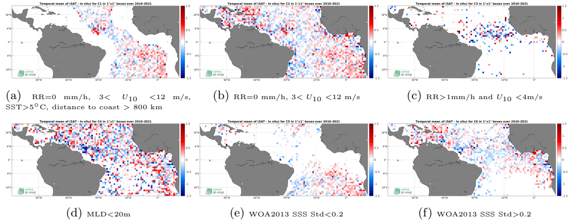
Figure 12: Temporal mean gridded over spatial boxes of size 1^\circ \times 1^\circ of \Delta SSS (SMOS SSS L2 v700 (ESA) - Argo) for 6 different subdatasets corresponding to: RR=0 mm/h, 3 < U_{10} < 12 m/s, SST > 5^\circ C , distance to coast > 800 km (a), RR=0 mm/h, 3 < U_{10} < 12 m/s (b), RR > 1 mm/h and U_{10} < 4 m/s (c), MLD < 20 m (d), WOA2013 SSS Std < 0.2 (e), WOA2013 SSS Std > 0.2 (f).
