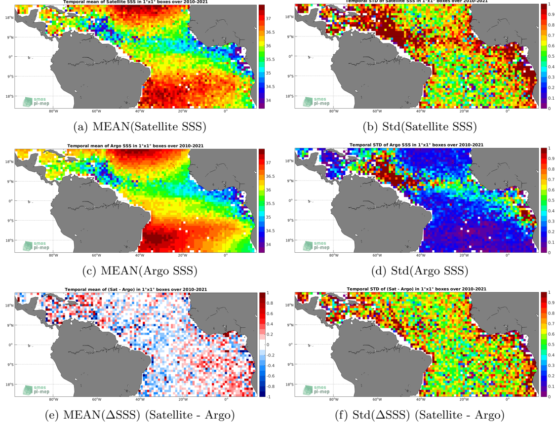
Figure 6: Temporal mean (left) and Std (right) of SSS from SMOS SSS L2 v700 (ESA) (top), Argo (middle), and of \Delta\text{SSS} (Satellite - Argo). Only match-up pairs are used to generate these maps.
