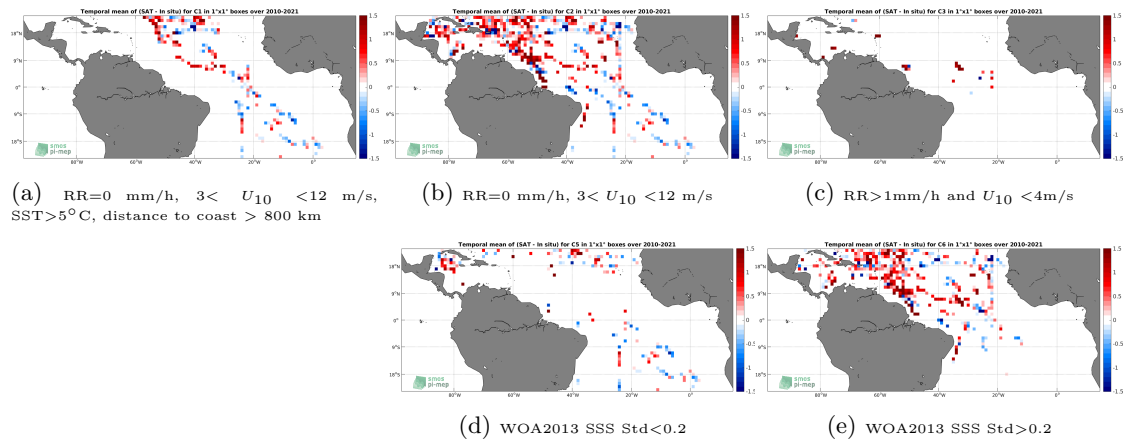
Figure 12: Temporal mean gridded over spatial boxes of size 1^\circ \times 1^\circ of \Delta SSS (SMOS SSS L2 v662 (ESA) - TSG (SAMOS)) for 5 different subdatasets corresponding to:RR=0 mm/h, 3 < U_{10} < 12 m/s, SST >5^\circ\text{C} , distance to coast > 800 km (a), RR=0 mm/h, 3 < U_{10} < 12 m/s (b), RR >1 mm/h and U_{10} < 4 m/s (c), WOA2013 SSS Std <0.2 (d), WOA2013 SSS Std >0.2 (e).
