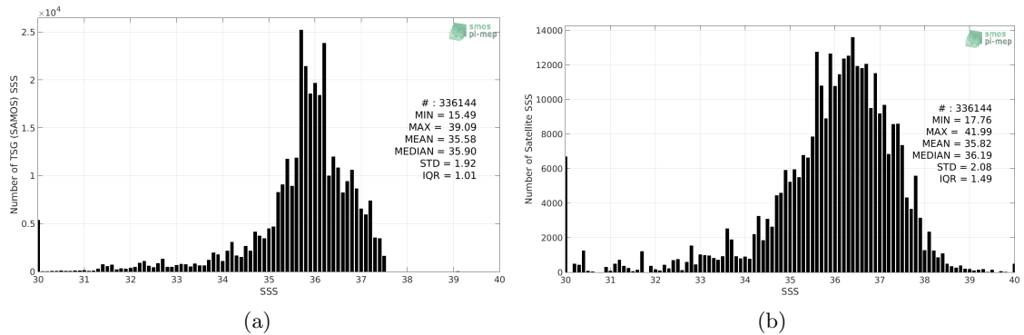
Figure 2: Histograms of SSS from TSG (SAMOS) (a) and SMOS SSS L2 v662 (ESA) (b) considering all match-up pairs per bins of 0.1 over the Tropical Atlantic Ocean Pi-MEP region and for the full satellite product period.
