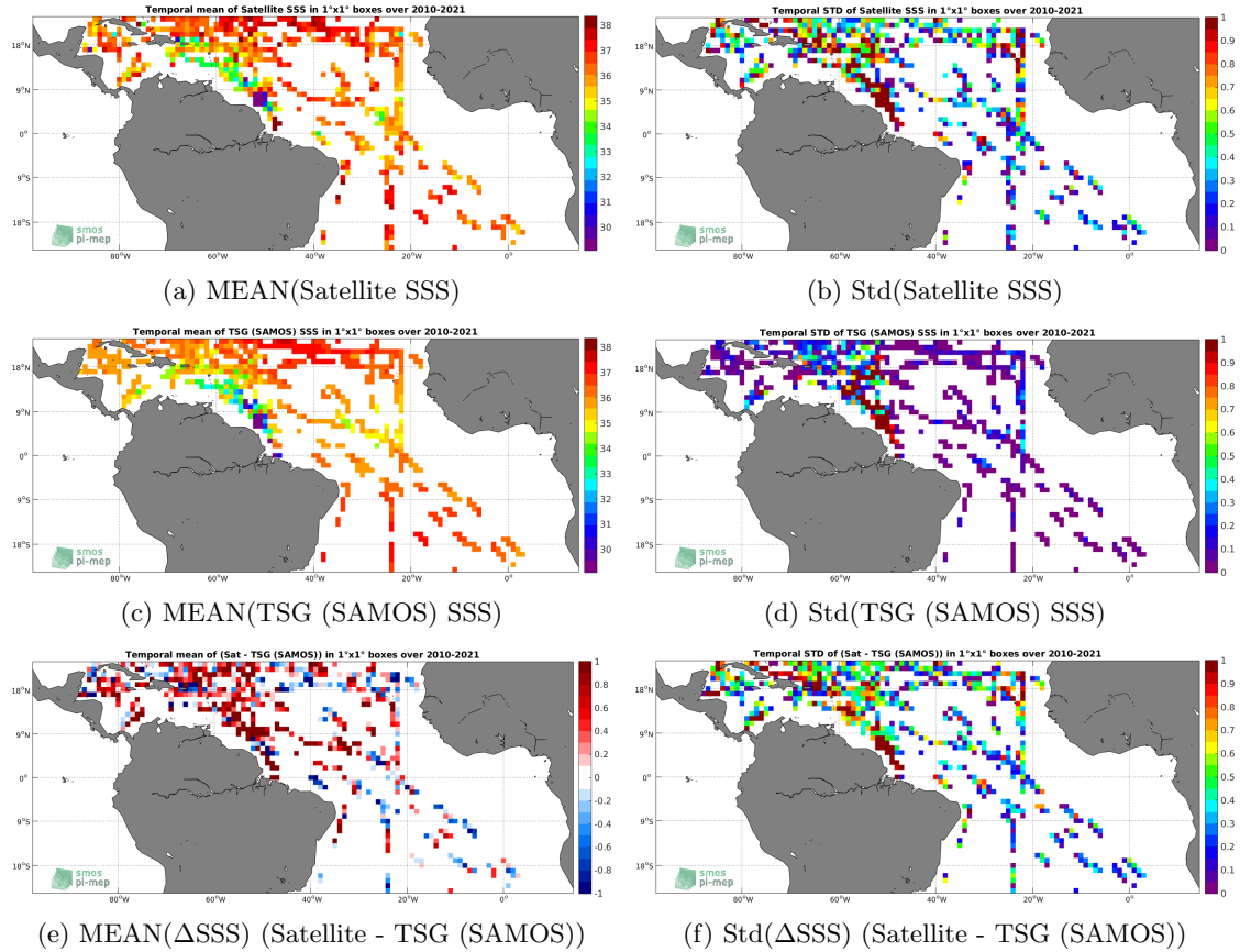
Figure 6: Temporal mean (left) and Std (right) of SSS from SMOS SSS L2 v662 (ESA) (top), TSG (SAMOS) (middle), and of \Delta SSS (Satellite - TSG (SAMOS)). Only match-up pairs are used to generate these maps.
