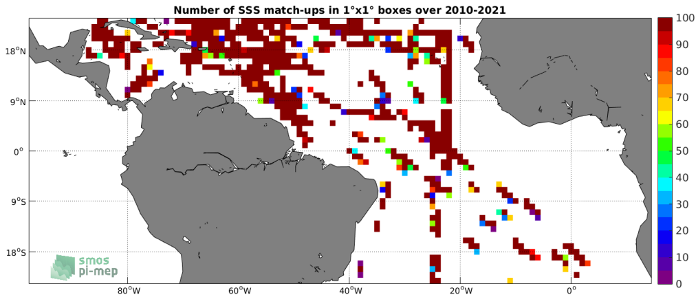
Figure 4: Number of SSS match-ups between TSG (SAMOS) SSS and the SMOS SSS L2 v662 (ESA) SSS product for the Tropical Atlantic Ocean Pi-MEP region over 1°x1° boxes and for the full satellite product period.
