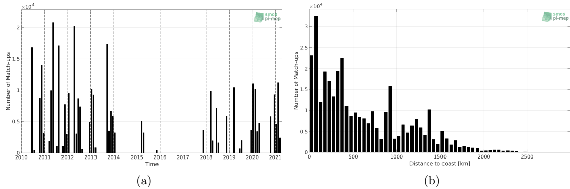
Figure 1: Number of match-ups between TSG (SAMOS) and SMOS SSS L2 v662 (ESA) SSS as a function of time (a) and as function of the distance to coast (b) over the Tropical Atlantic Ocean Pi-MEP region and for the full satellite product period.
